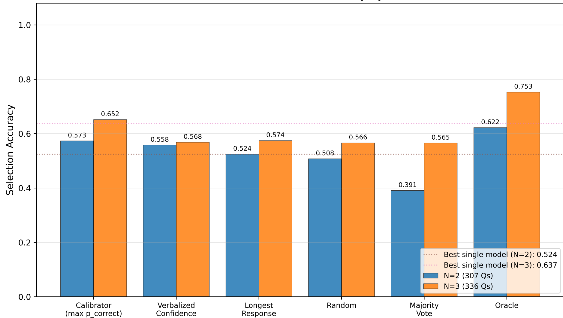
UC-B: Best-of-N Selection Accuracy by Method
