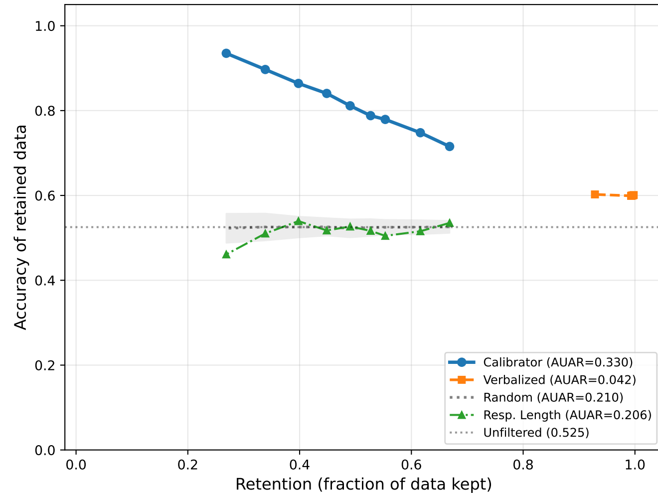
Qwen3.5 (N=573)
