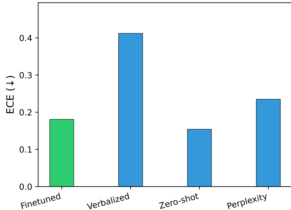
Expected Calibration Error
