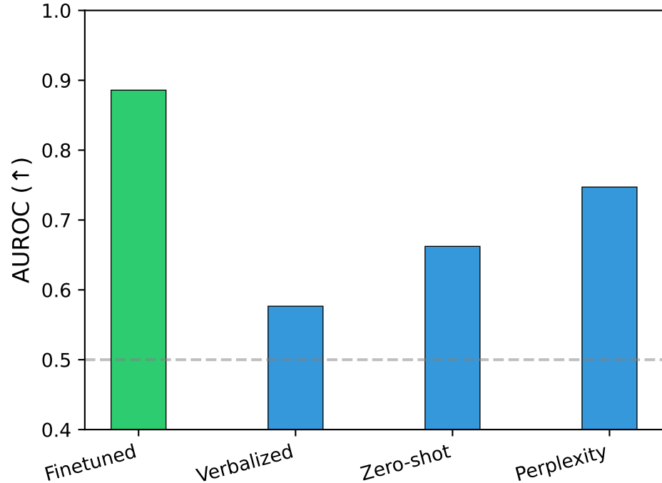
Area Under ROC Curve
