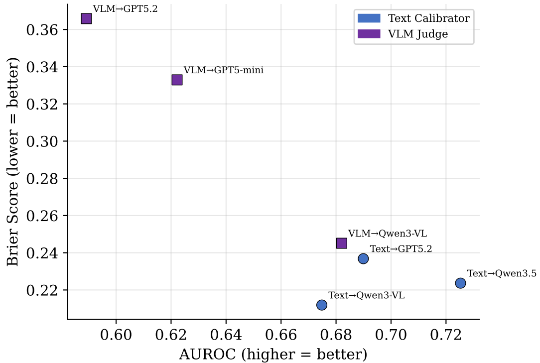
(b) Discrimination vs Calibration
