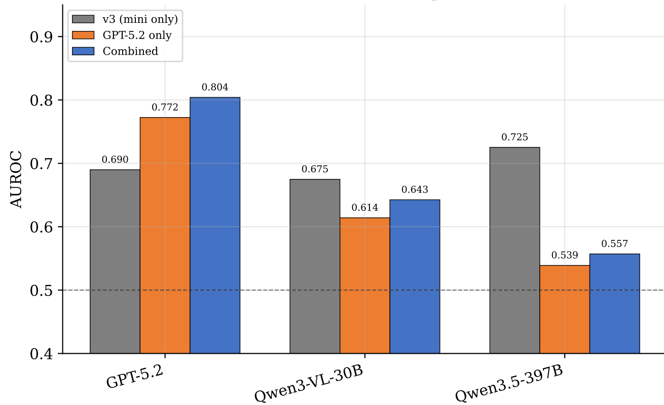
(a) Text Calibrator Comparison
