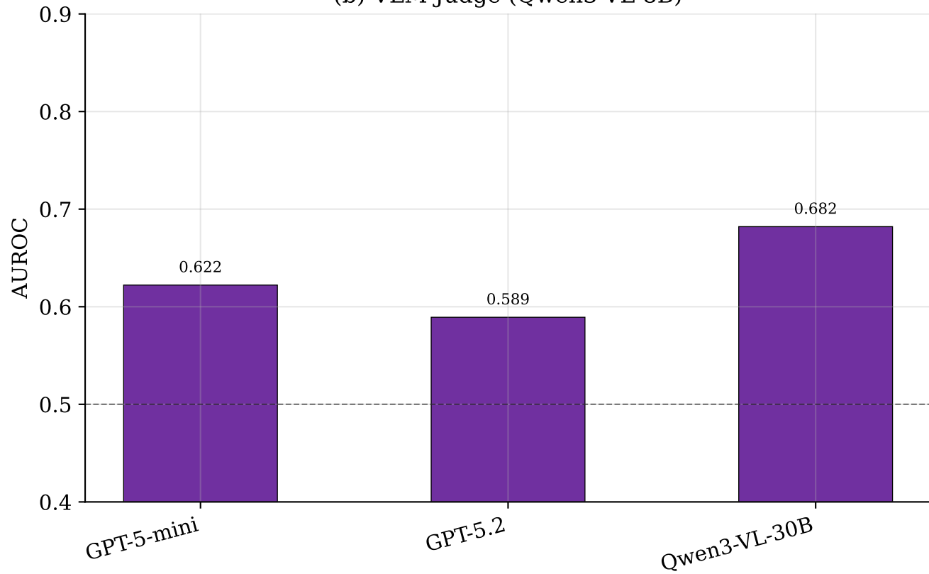
(b) VLM Judge (Qwen3-VL-8B)
