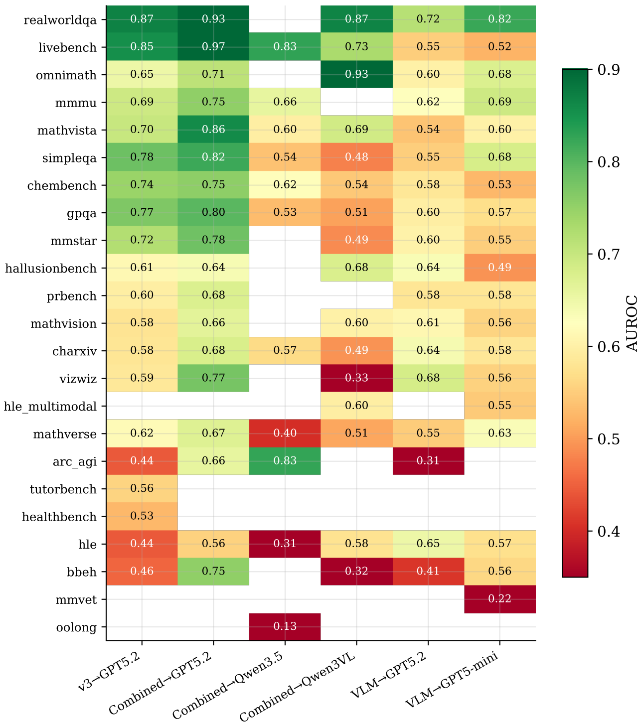
Per-Benchmark AUROC Across Models
