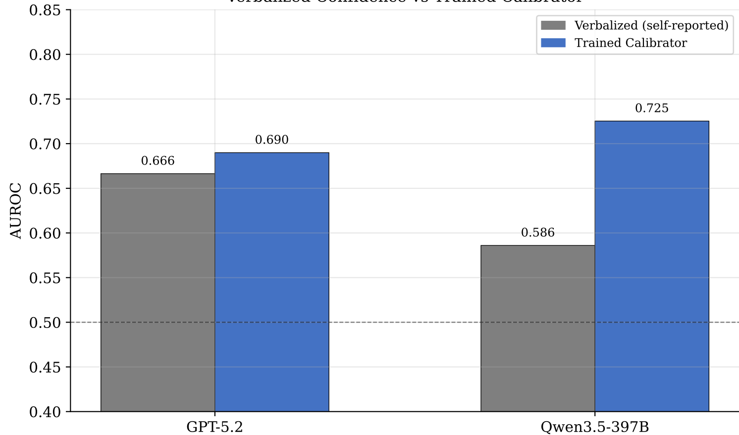
Verbalized Confidence vs Trained Calibrator
