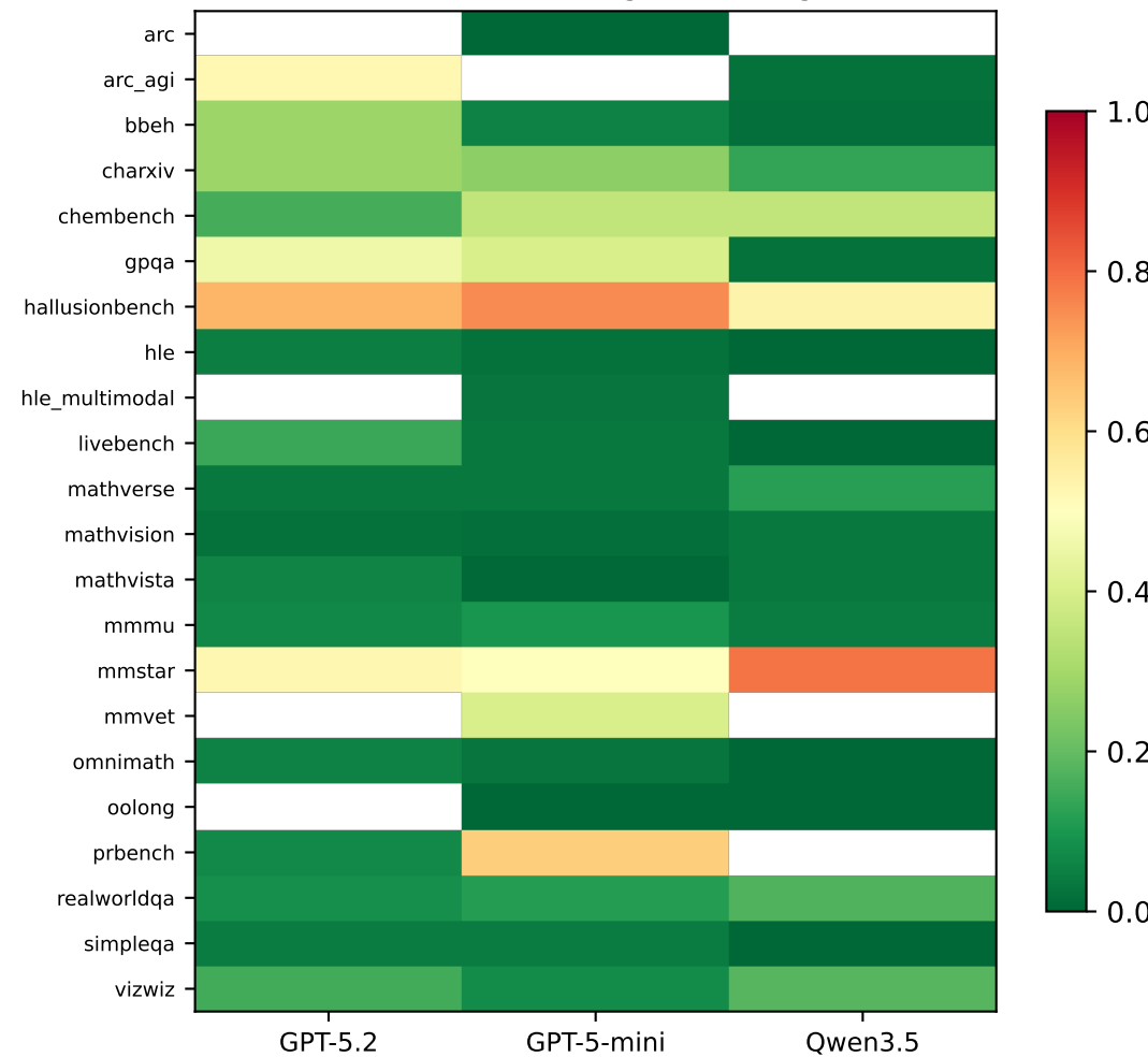
Overconfident Error Rate ( P > 0.7 but wrong / all wrong)
