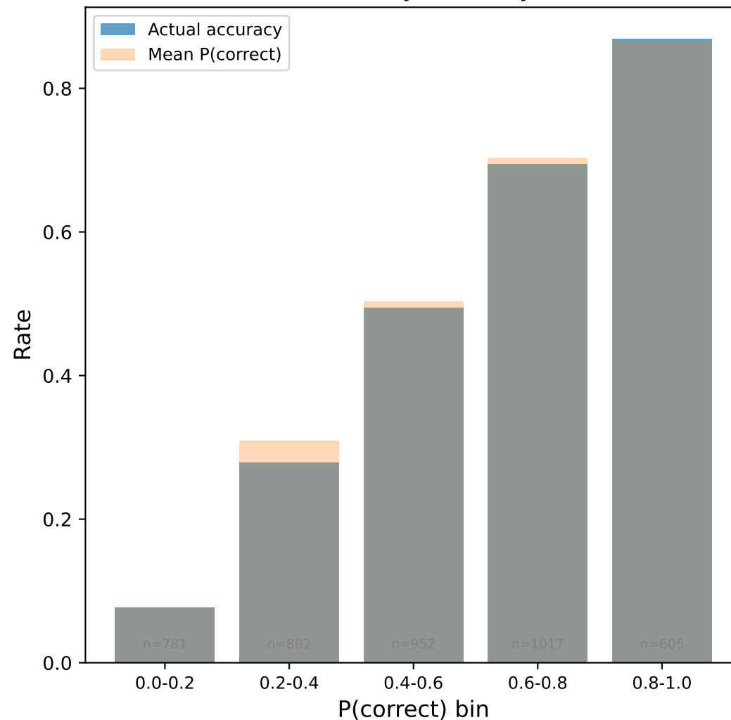
Calibration by Difficulty Bin
