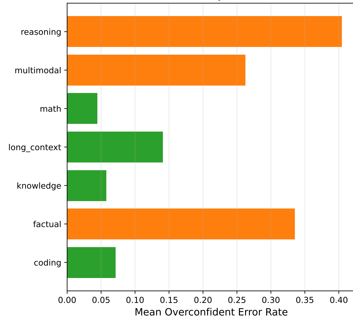
Weakness by Domain
