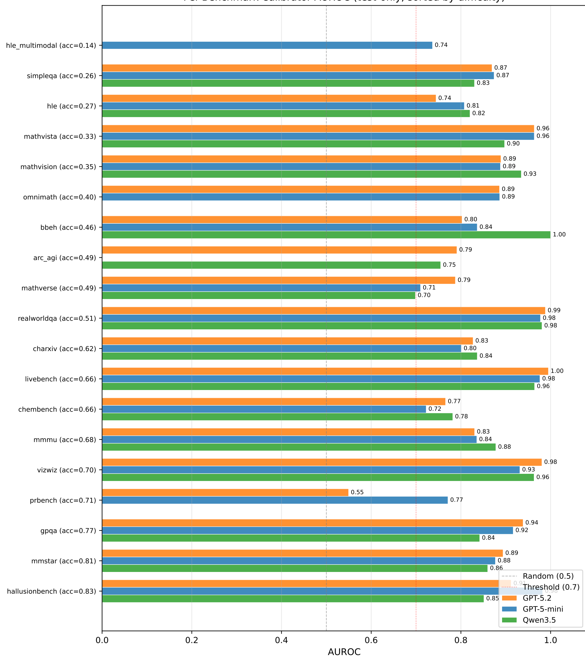
Per-Benchmark Calibrator AUROC (test-only, sorted by difficulty)
