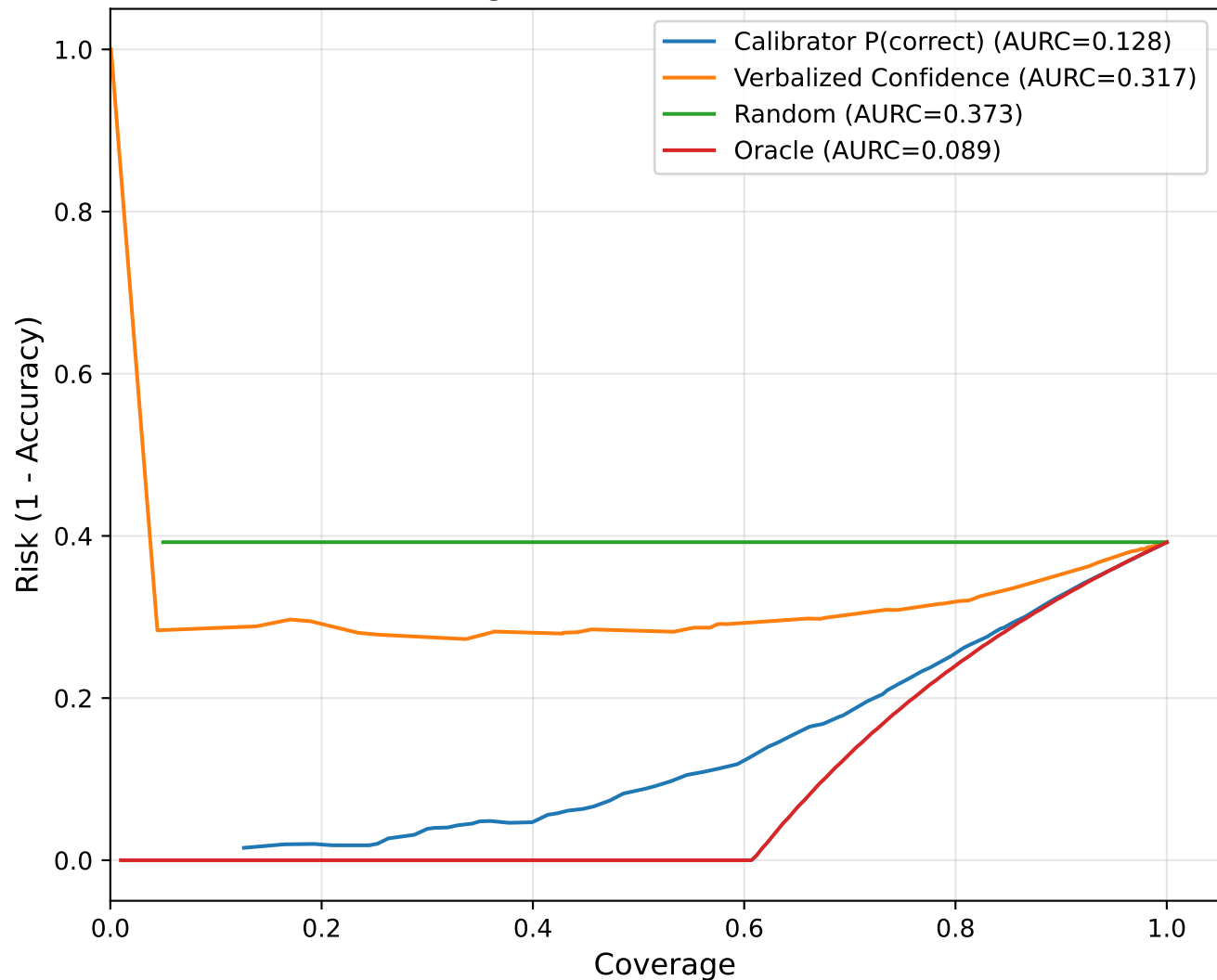
Risk-Coverage Curve — GPT-5.2 (cross-model)
