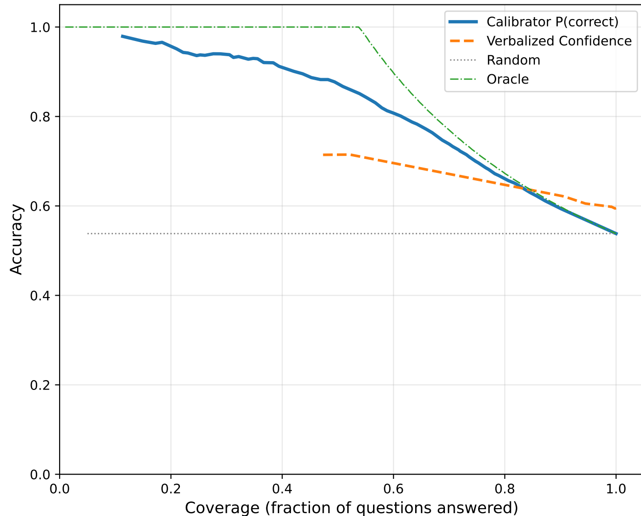
Selective Prediction — Qwen3.5 (cross-model)
