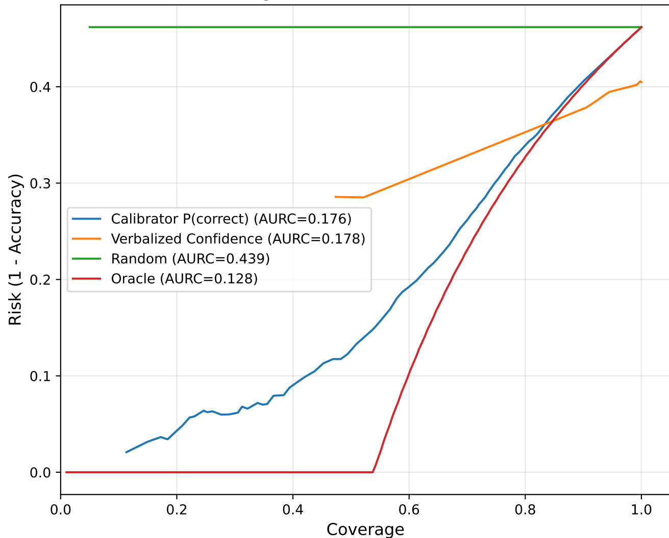
Risk-Coverage Curve — Qwen3.5 (cross-model)
