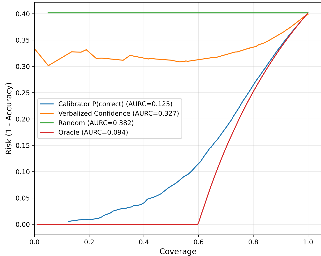
Risk-Coverage Curve — GPT-5.2 (cross-model)
