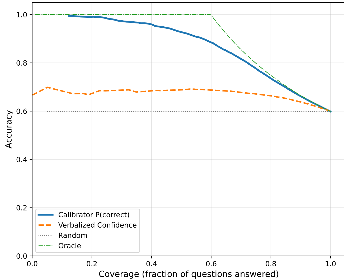
Selective Prediction — GPT-5.2 (cross-model)
