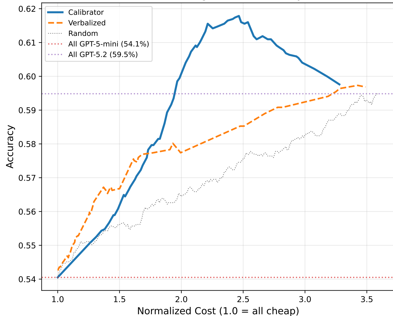
Model Routing: Cost vs Accuracy
