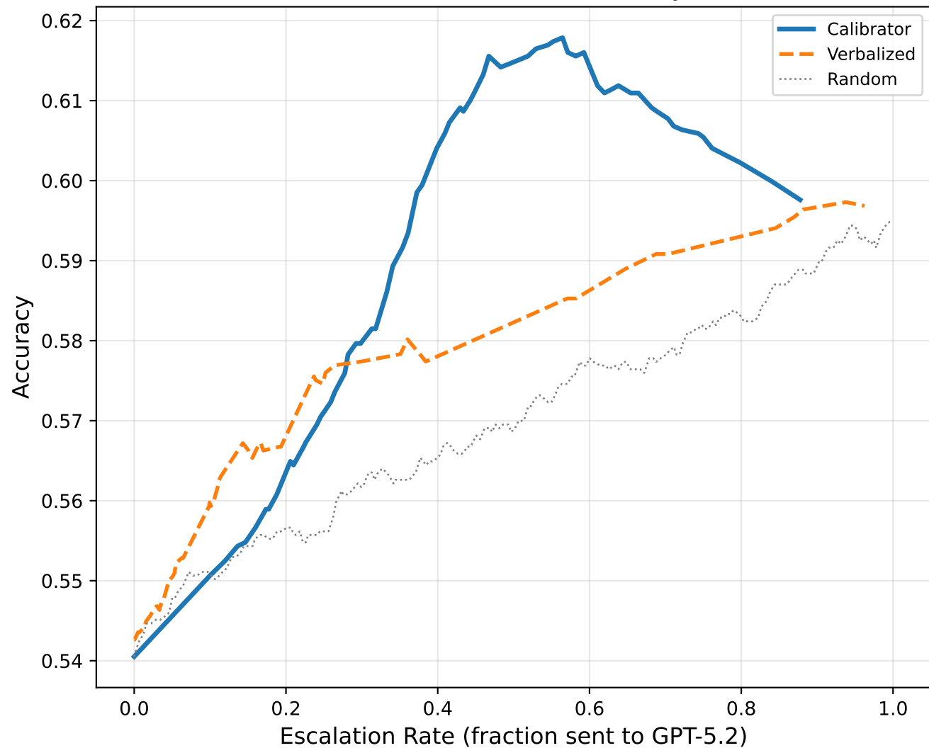
Escalation Rate vs Accuracy
