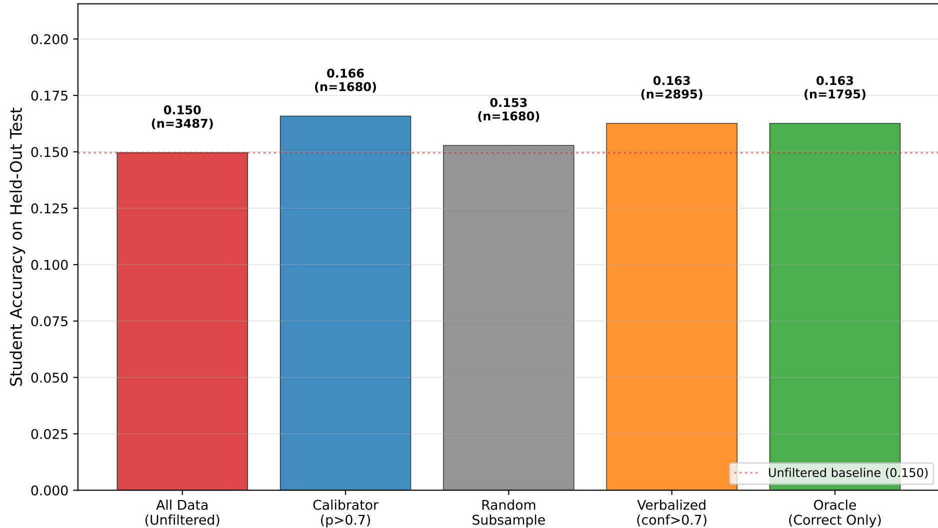
UC-C Stage 2: Student Accuracy by Training Data Filter
