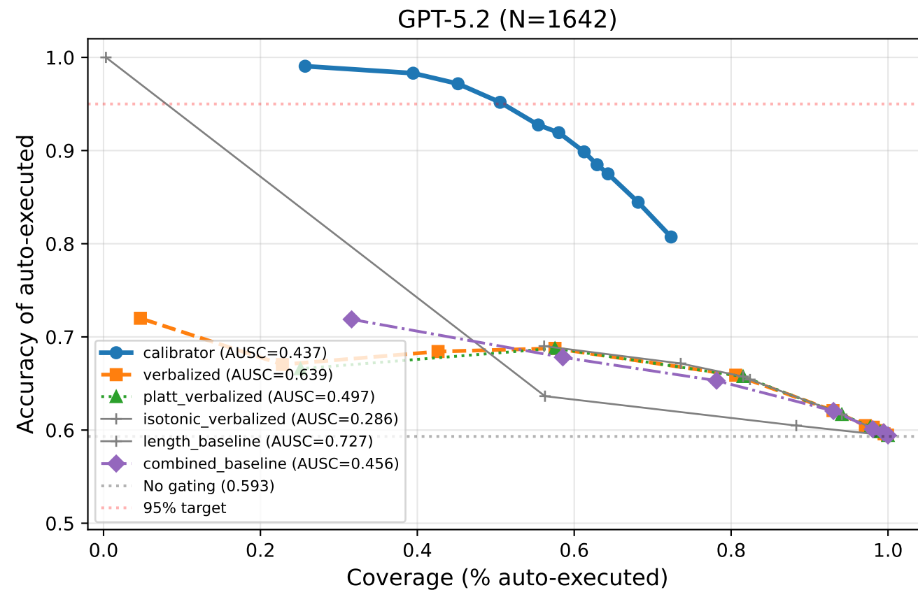
UC-F: Confidence-Gated Actions — Coverage vs Safety
