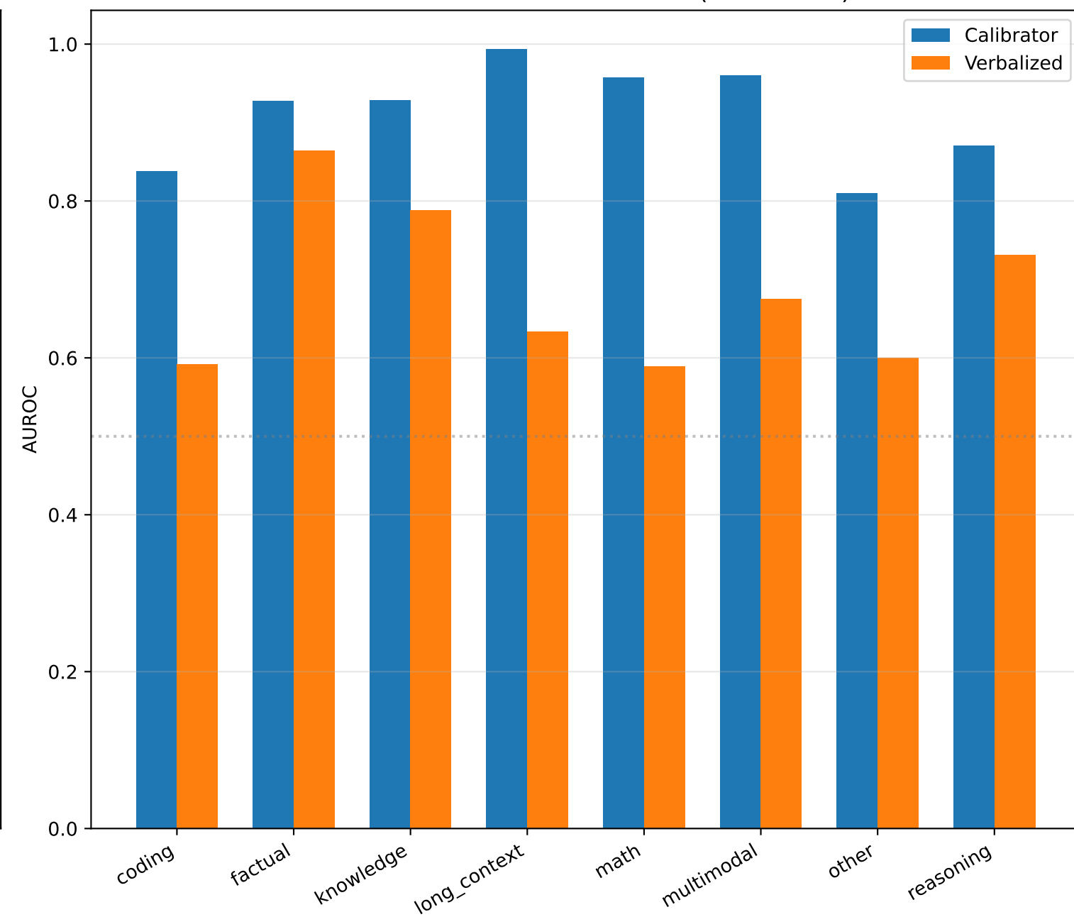
D. Method Comparison (GPT-5-mini)
