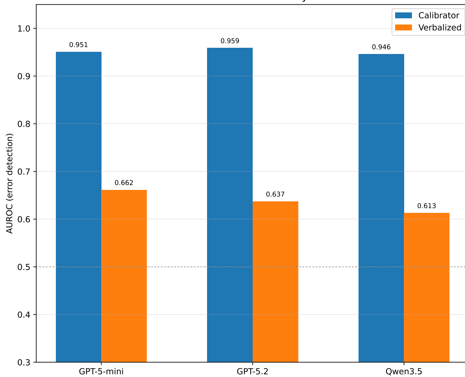
A. Error Detection AUROC by Method
