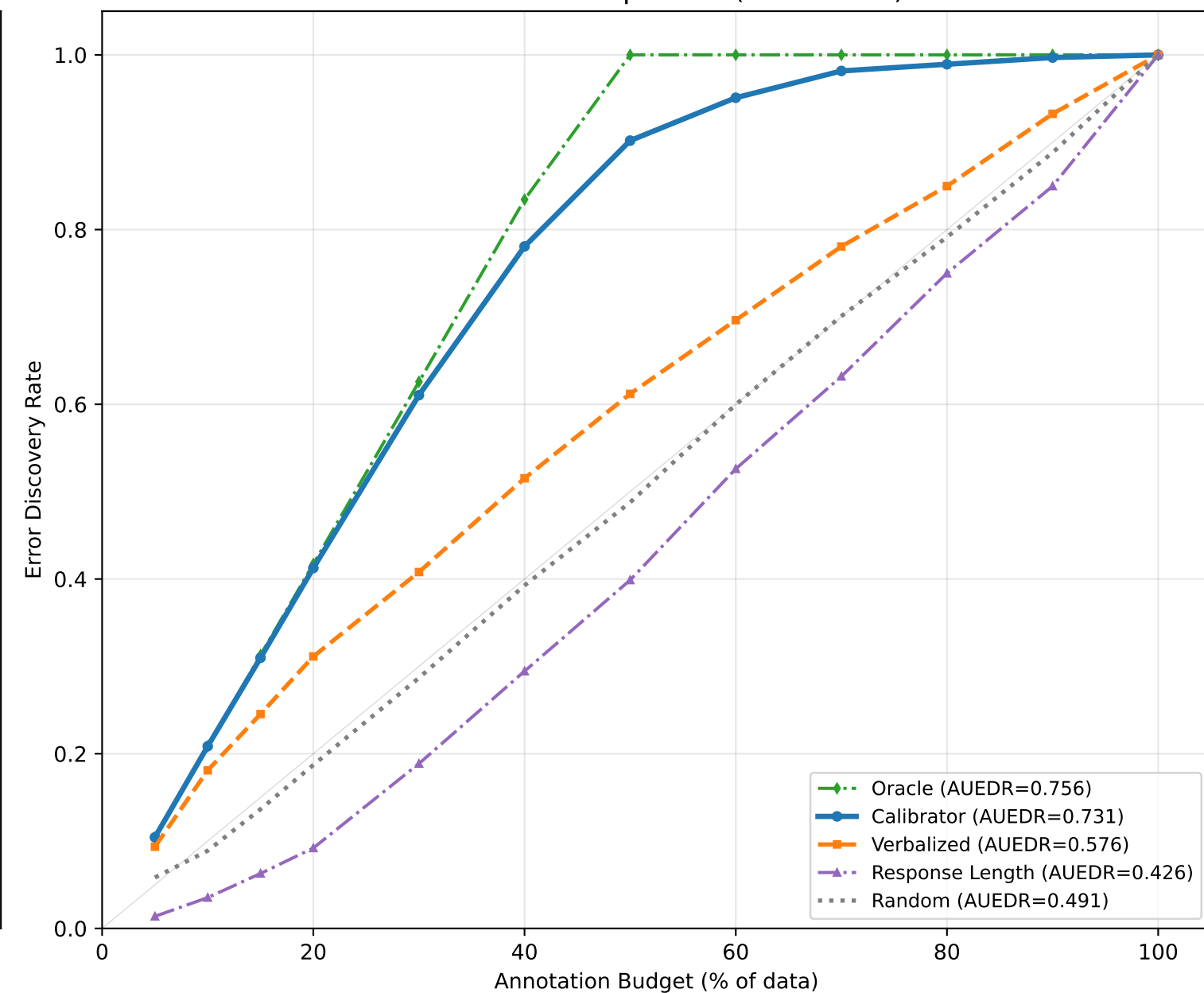
D. Method Comparison (GPT-5-mini)
