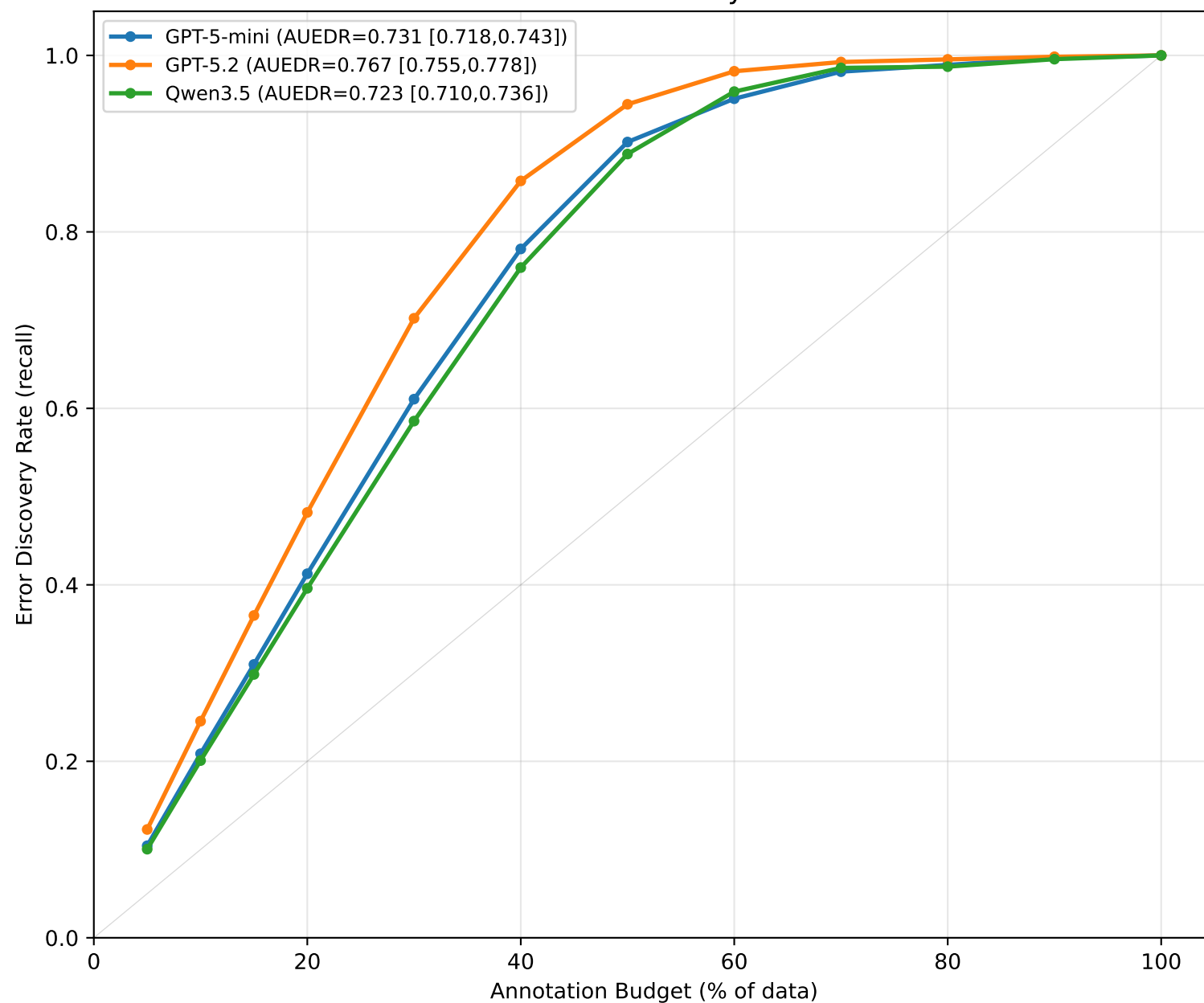
C. Annotation Efficiency: Calibrator
