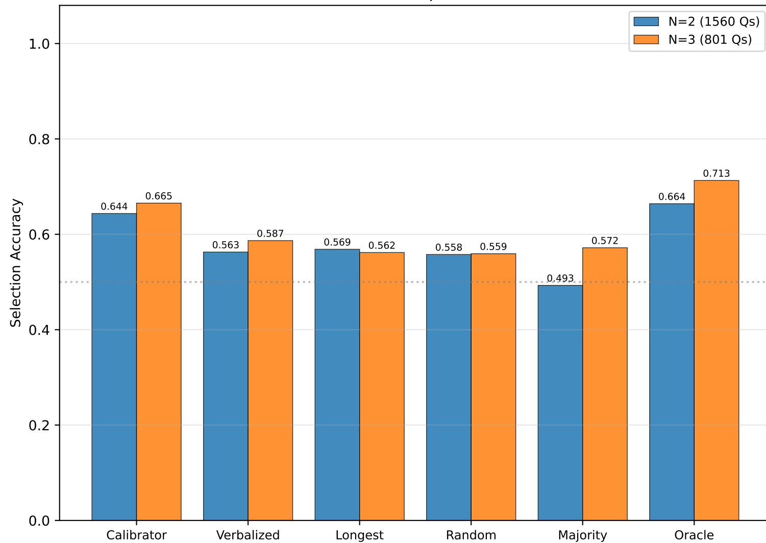
UC5: Best-of-N Response Selection
