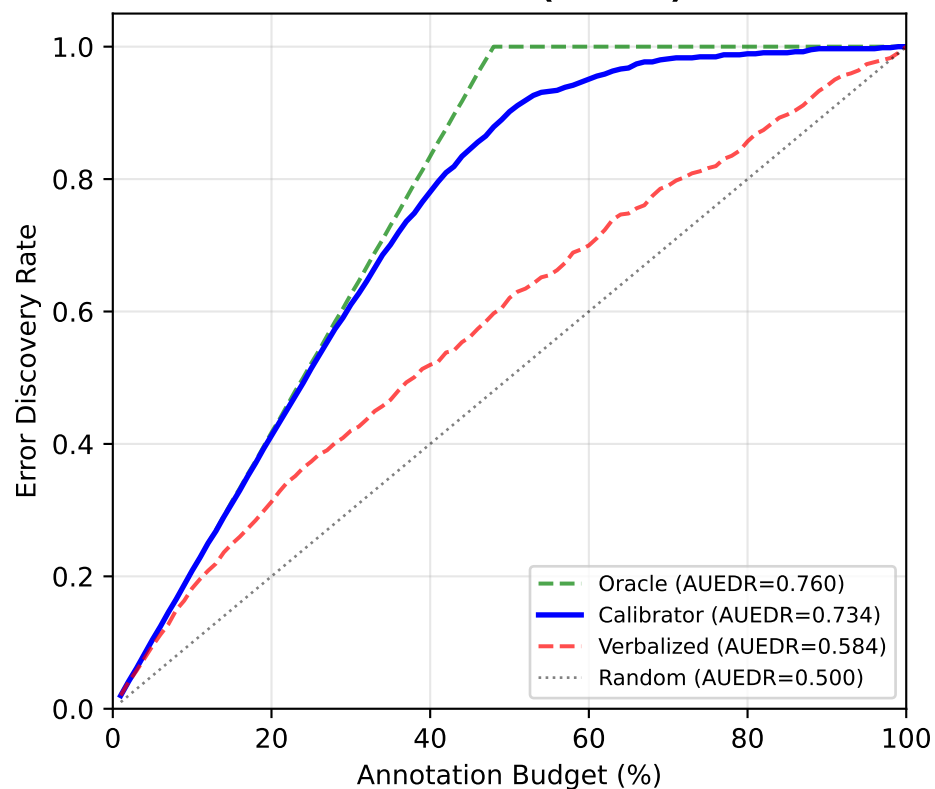
Qwen3.5 (cross-model)
