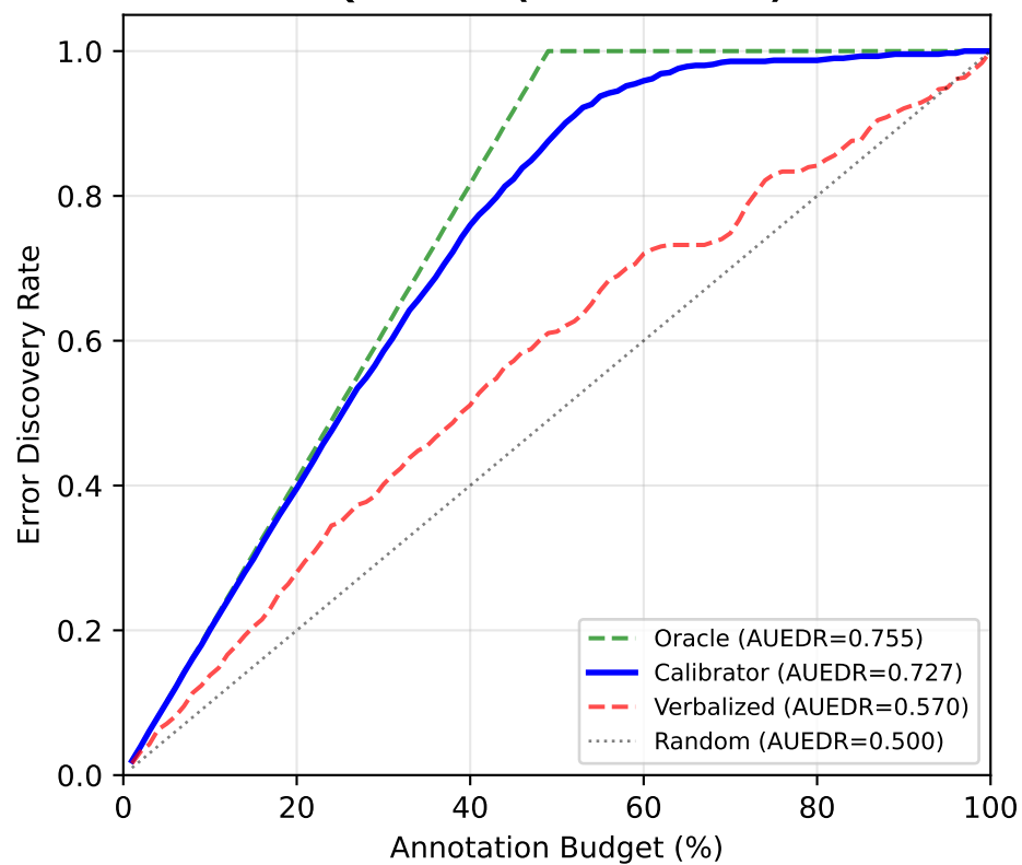
Qwen3.5 (cross-model)
