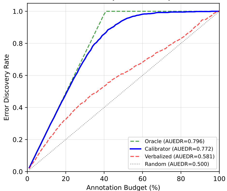
GPT-5.2 (cross-model)
