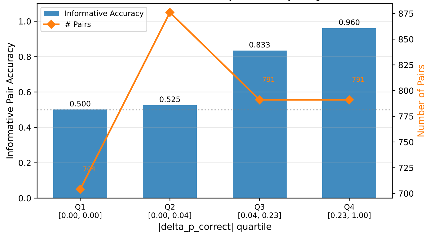
Informative Pairs: Accuracy & Count by Margin
