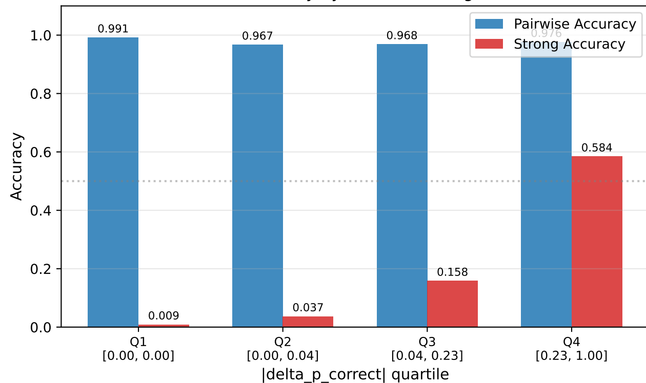
Pair Quality by Calibrator Margin
