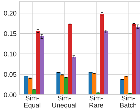
Biozero-MSE
