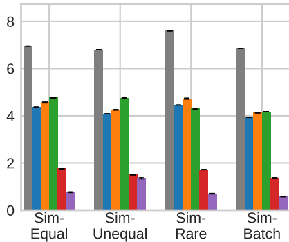
Overall MSE
