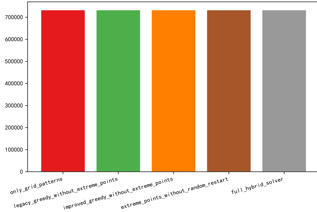
Total Profit
