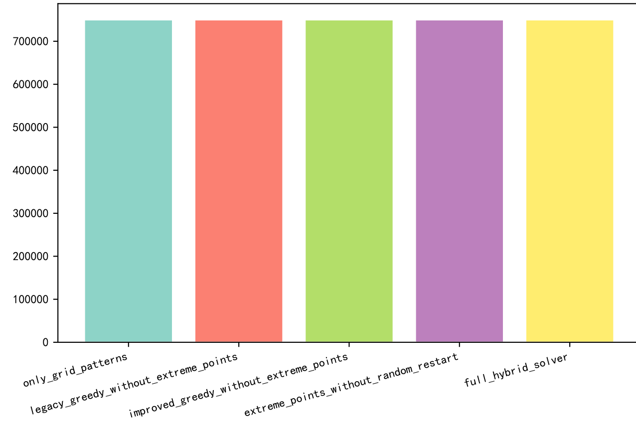
Runtime (seconds)
