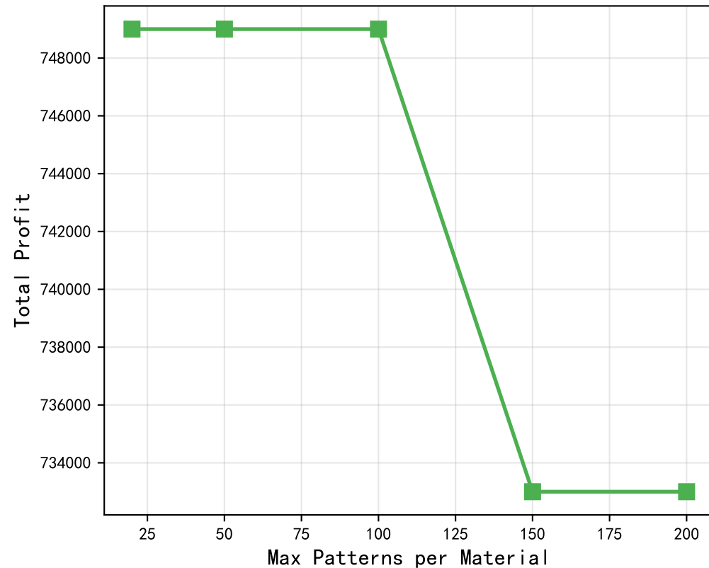
Profit vs Pattern Count
