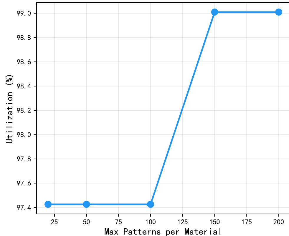
Utilization vs Pattern Count
