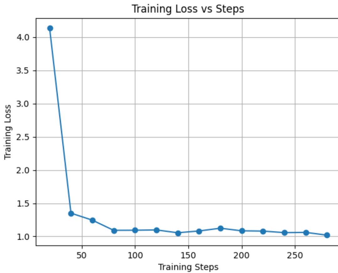
Figure 6: Training loss curve over the 1-epoch fine-tuning run. The loss fluctuates over the steps but maintains an overall downward trend, indicating effective learning and adaptation to the domain.
