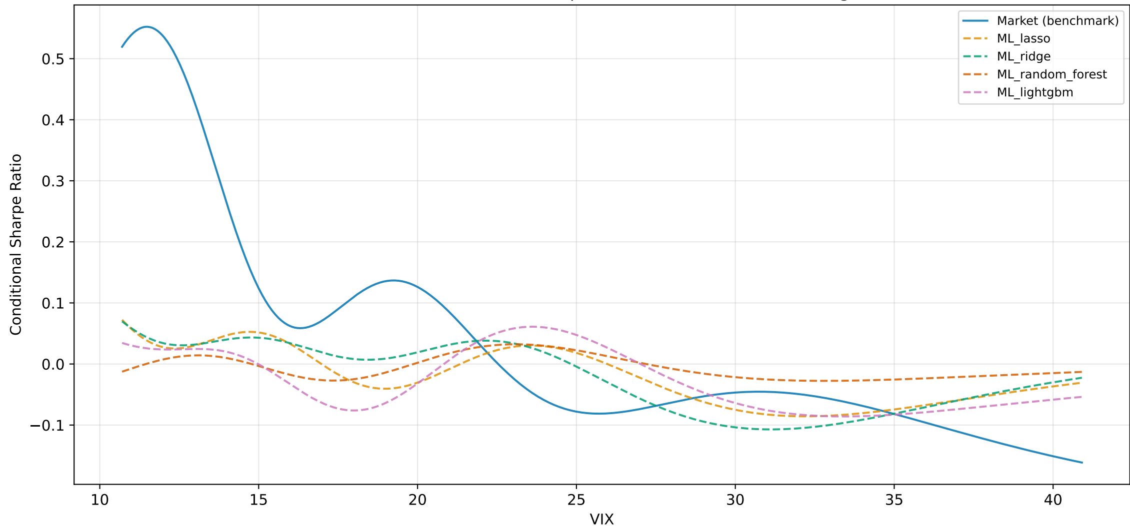
Estimated Conditional Sharpe Ratios: Market vs ML Strategies
