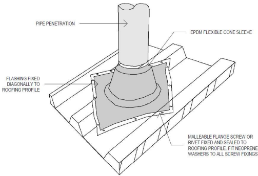
2 ROOF PIPE PENETRATION DETAIL
