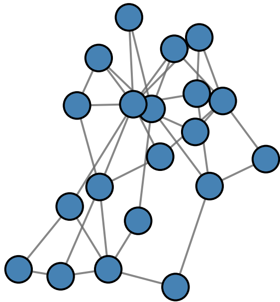
(b) Barabási-Albert
