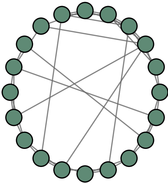
(c) Watts-Strogatz
