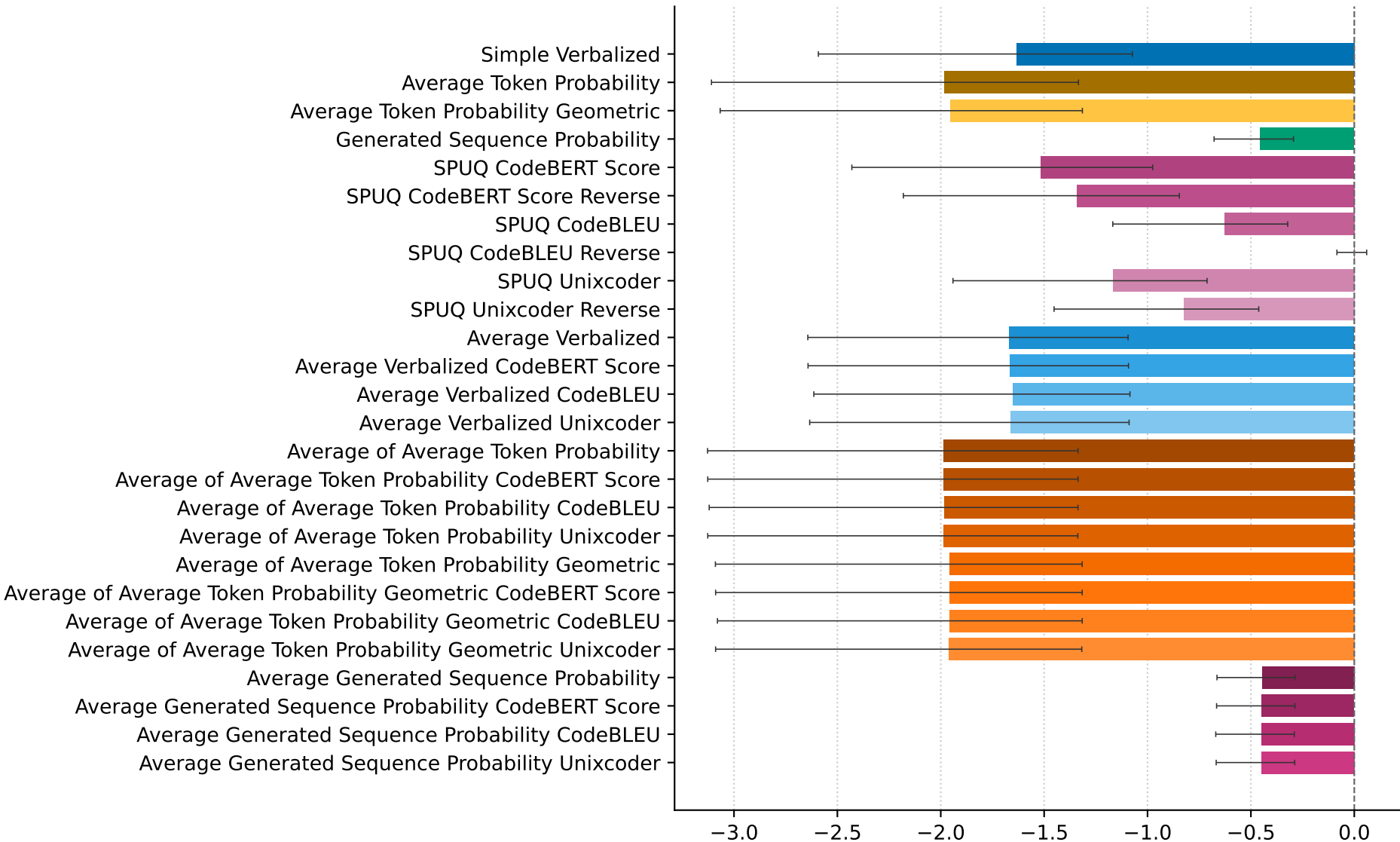
Skill score (higher is better)
