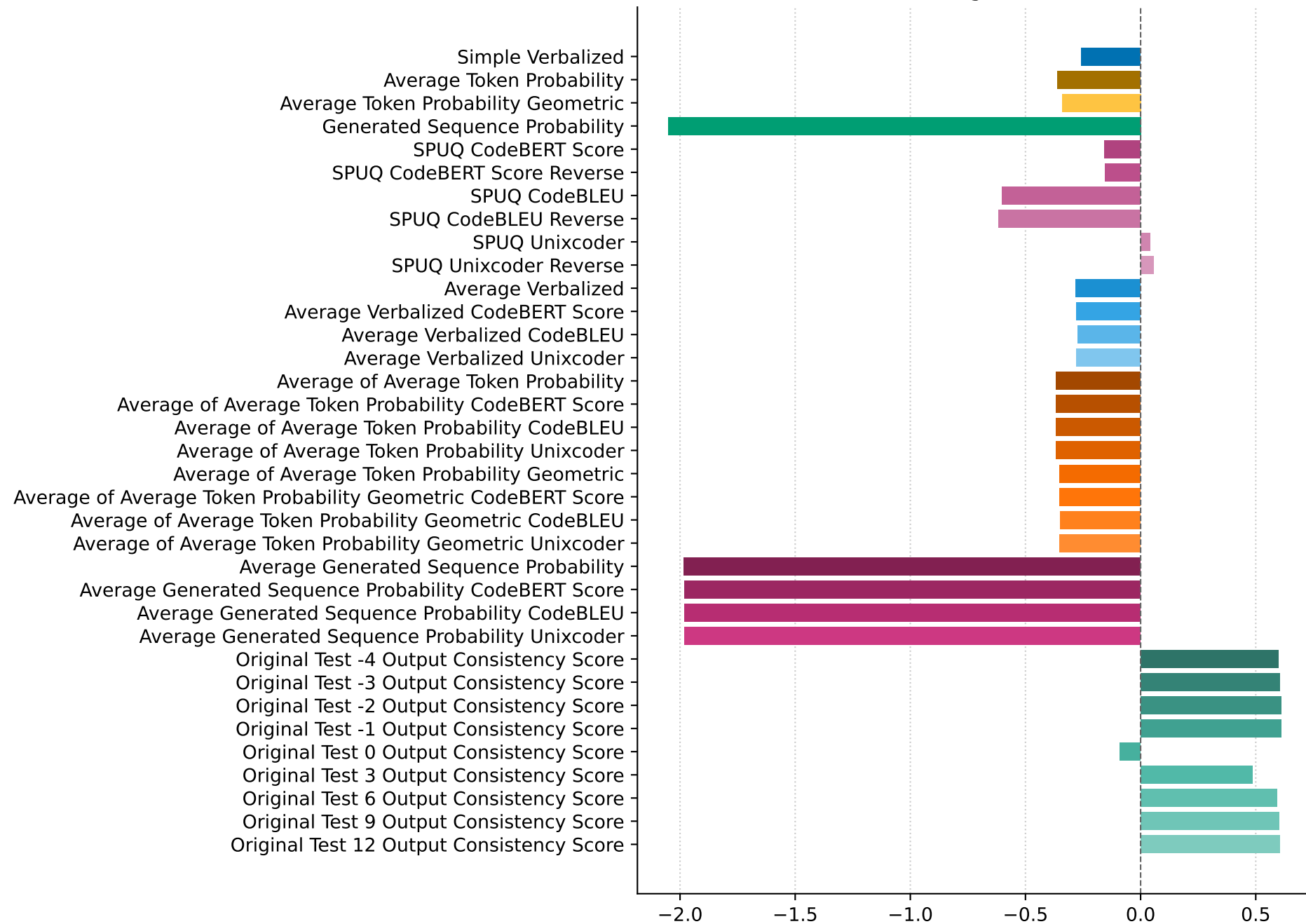
Skill score (higher is better)
