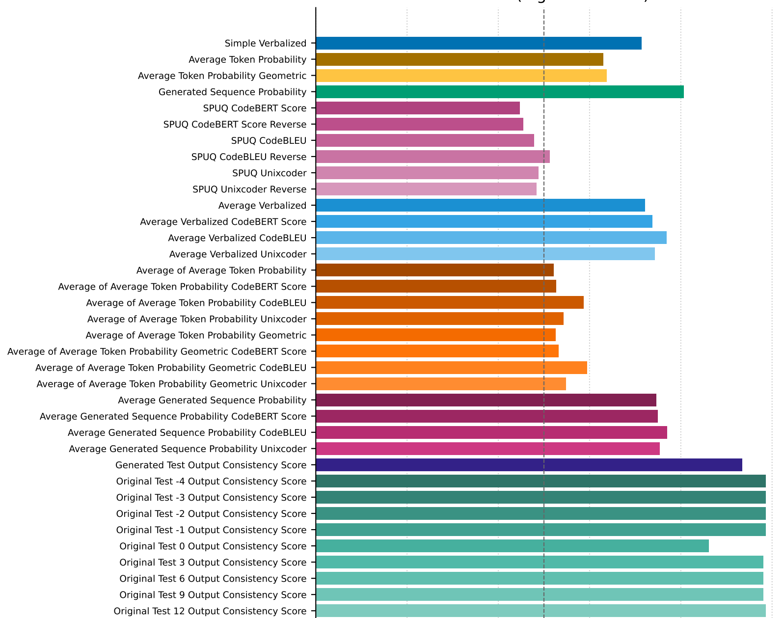
AUROC (higher is better)
