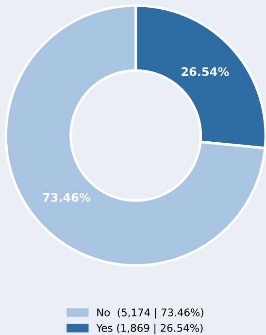
Churn Distribution
