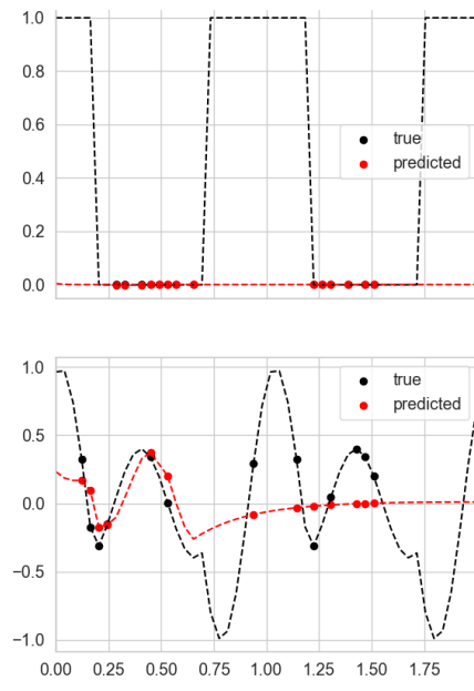
Neural CDE
