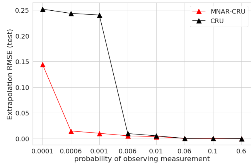
Model
