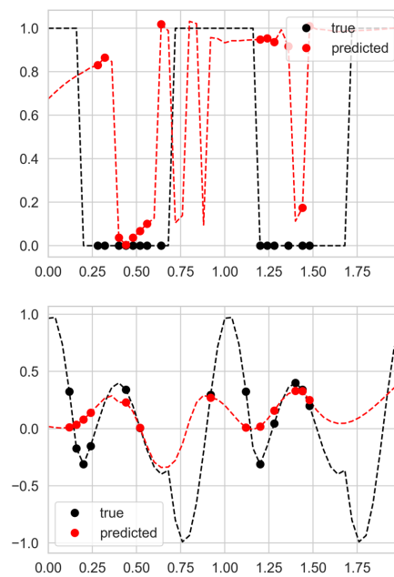
Neural CDE
