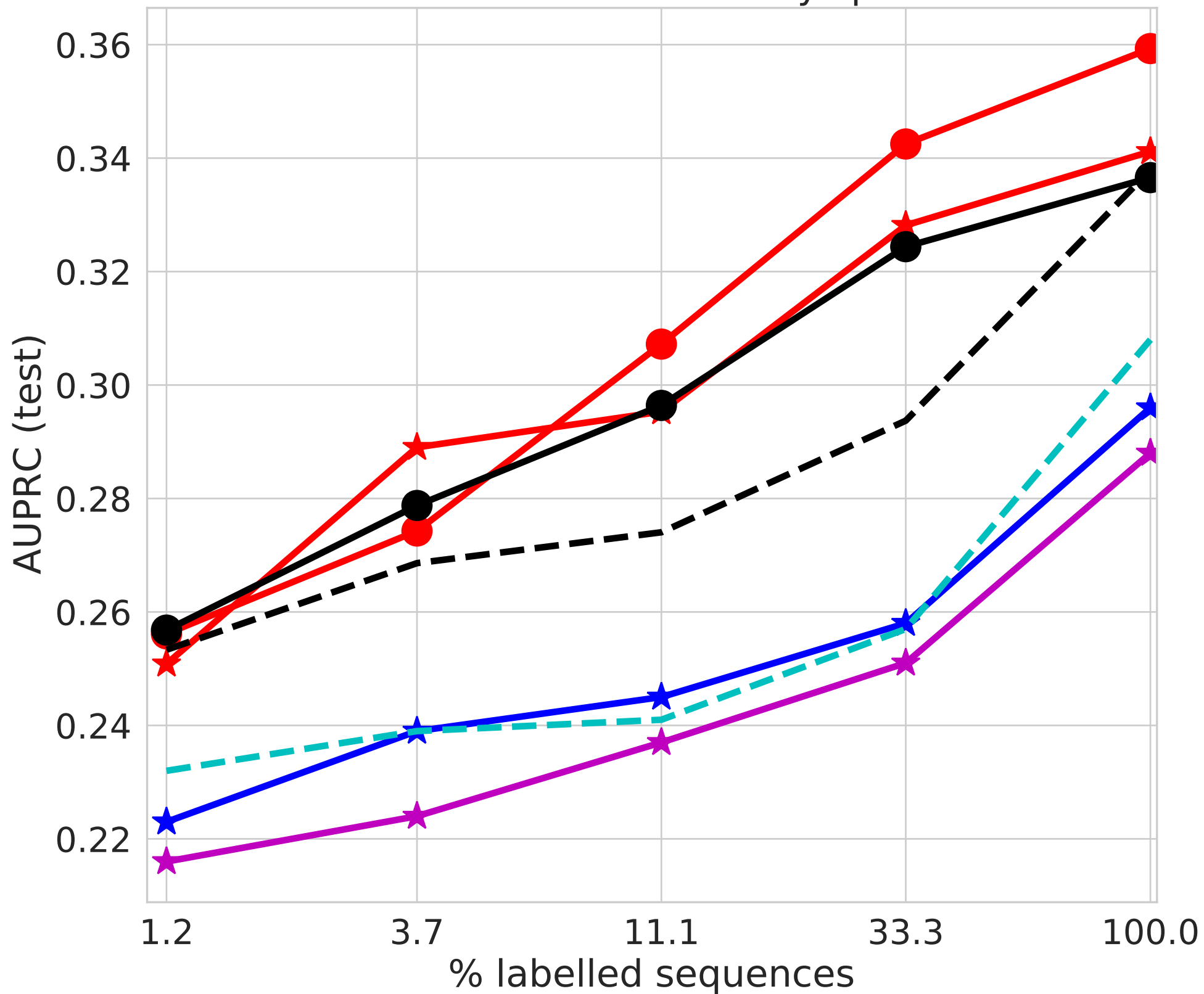
Performance for LOS > 5 days prediction
