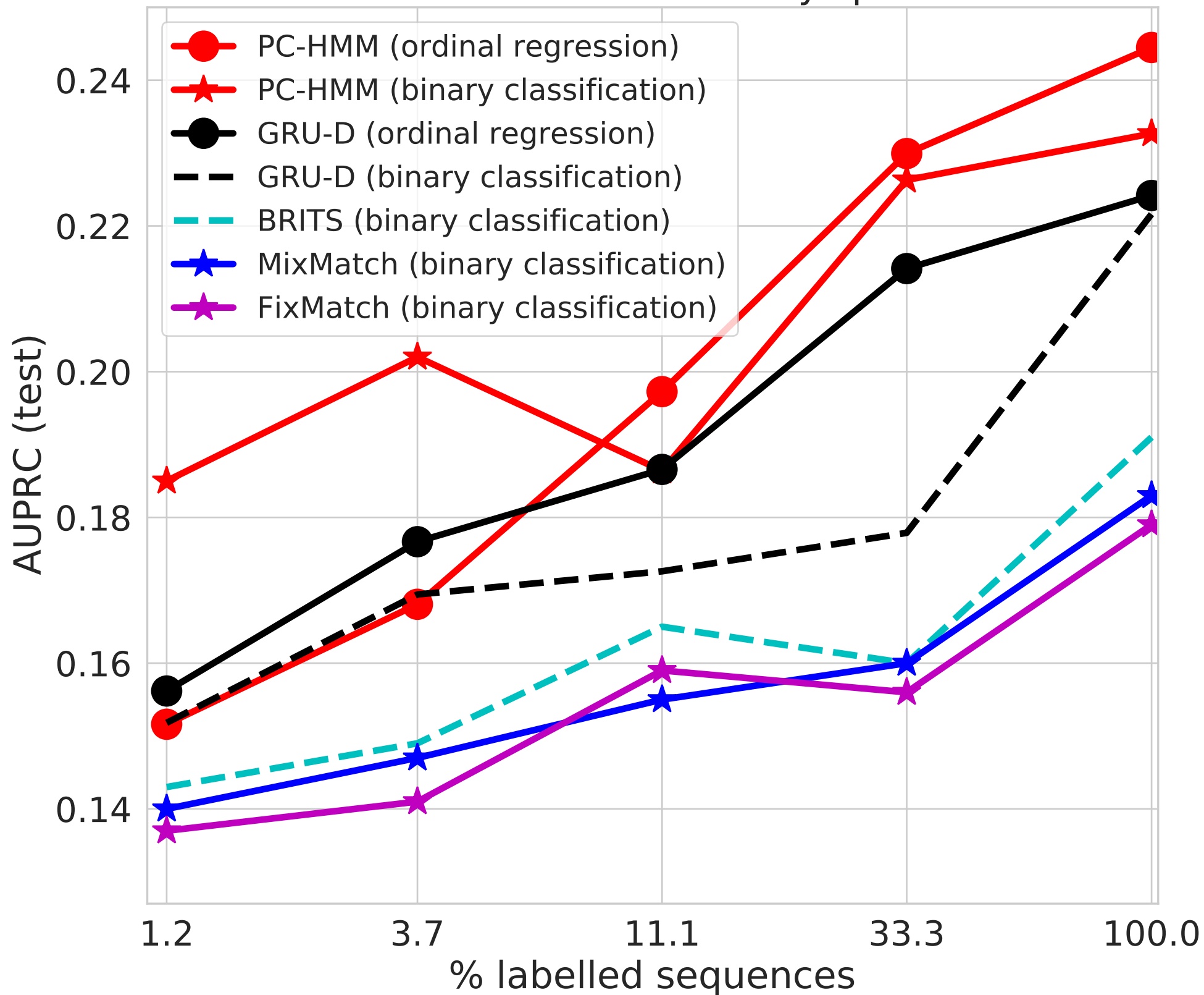
Performance for LOS > 7 days prediction
