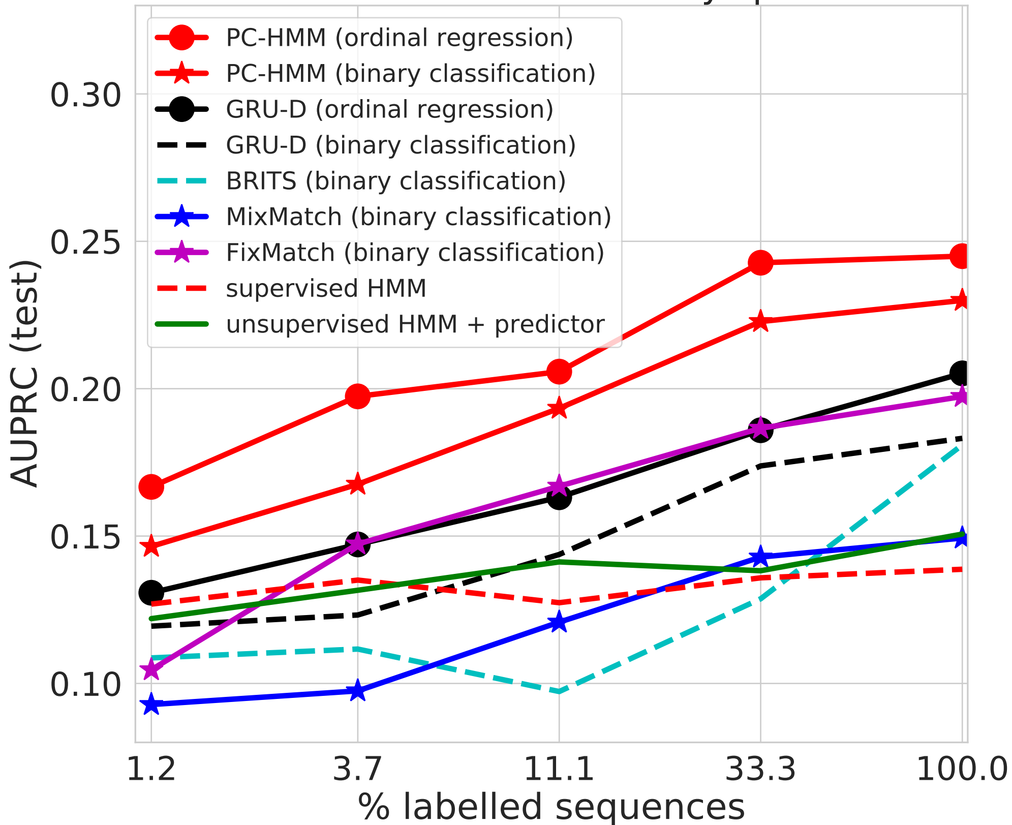
Performance for LOS > 11 days prediction
