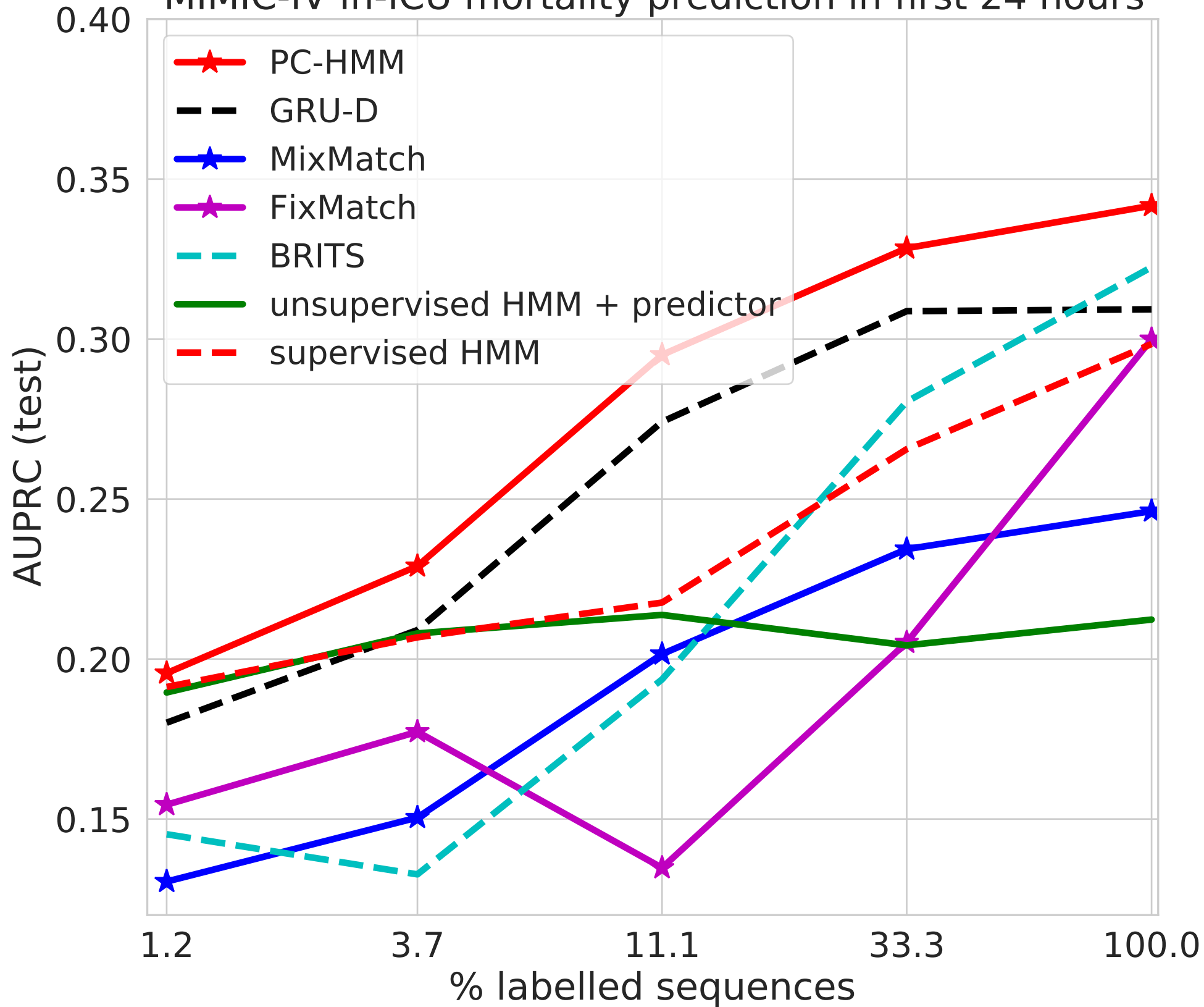
MIMIC-IV In-ICU mortality prediction in first 24 hours
