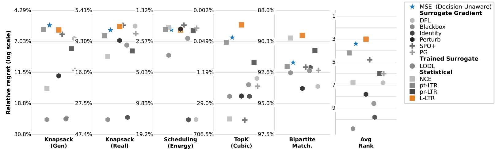
Benchmark re-run, Tasks with Limited Decision-Aware benefit, Relative regret % (best ↑)
