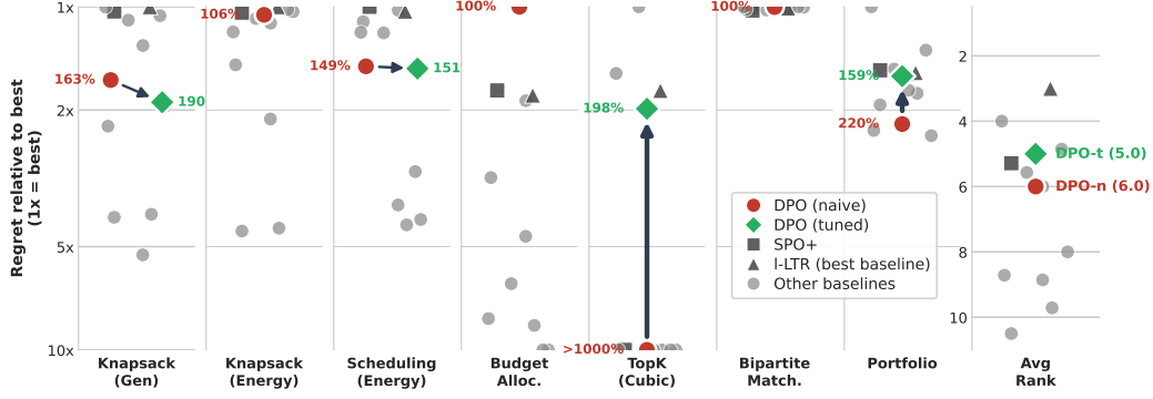
Figure 5.1: 7 task benchmark from Geng et al. Each column is a task. DPO: naive grid search vs. extra tuning.
