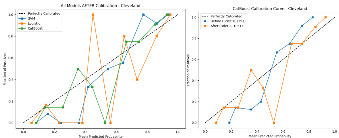
Figure 4.2. Calibration Curves - Cleveland
