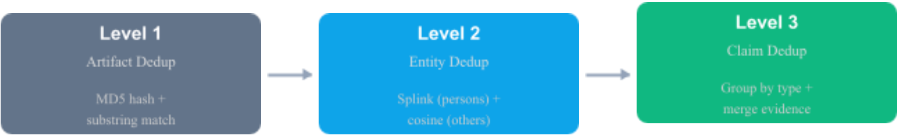
Figure 3 - Three-level deduplication pipeline
