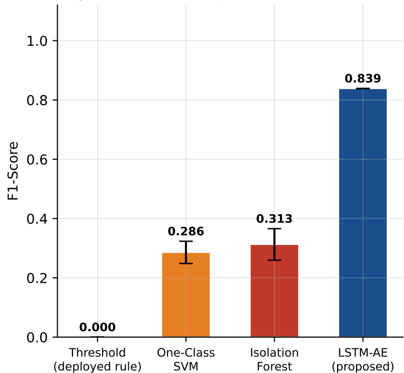
Early fire detection (pre-smoke) — F1-Score
