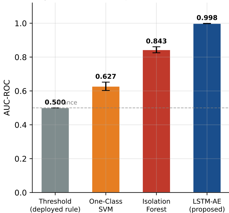
Early fire detection (pre-smoke) — AUC-ROC
