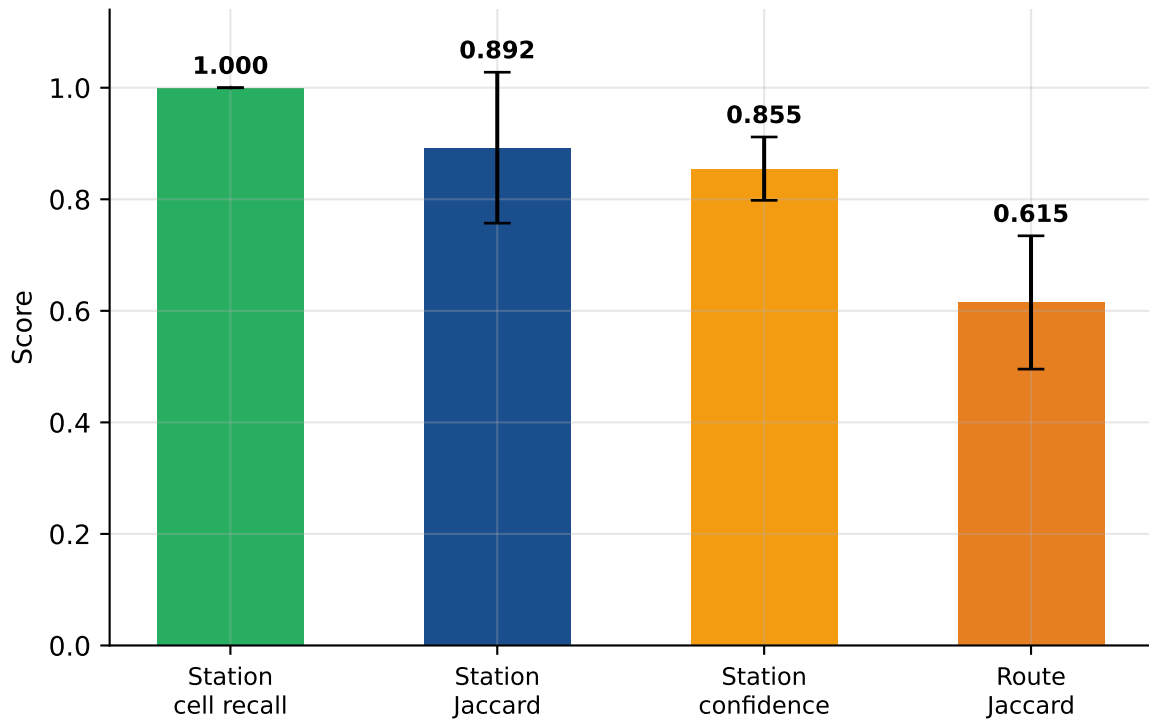
Model ⑤ — recovery of the configured station and route (20 runs, 10 shifts each)
