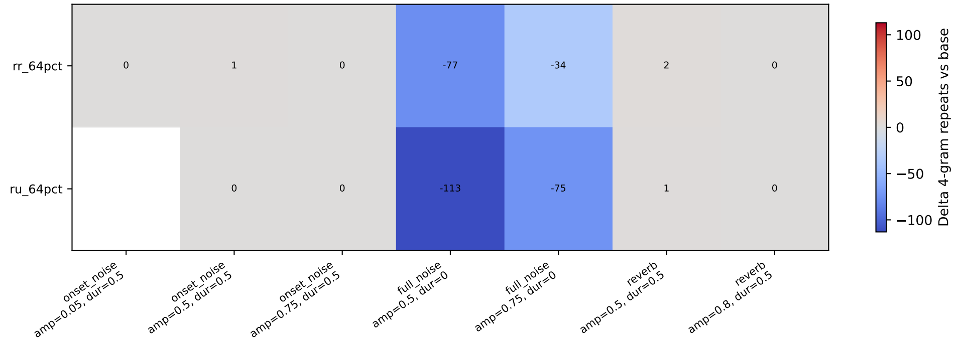
Stress response matrix: Delta 4-gram repeats vs base
