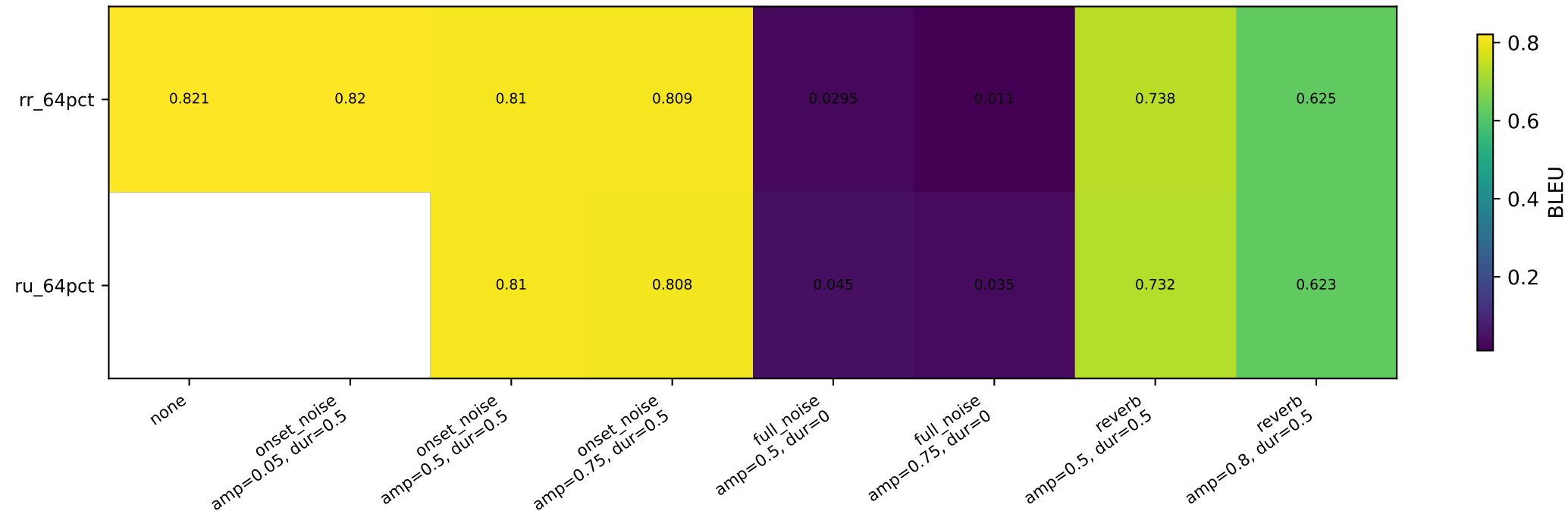
Stress response matrix: BLEU
