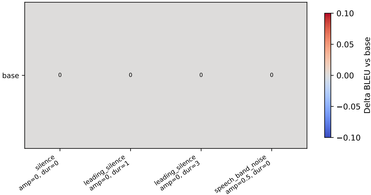
Stress response matrix: Delta BLEU vs base
