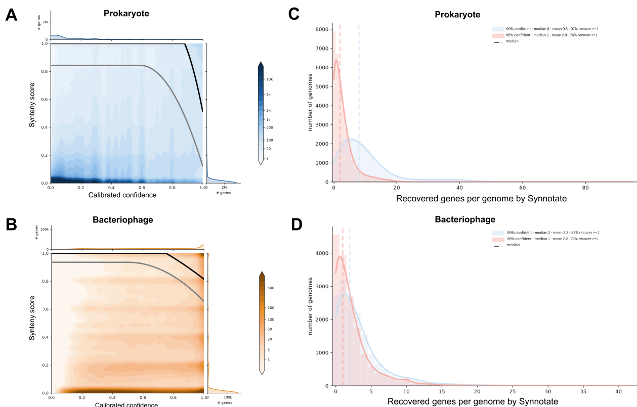
Figure S3. Annotation of the dark proteome of prokaryotic and bacteriophage datasets. (A) Synnotate calibrated confidence and Synteny score of dark genes in Prokaryote dataset. (B) Synnotate calibrated confidence and Synteny score of dark genes in Bacteriophage dataset. (C) Number of genes confidently annotated by Synnotate per genome in Prokaryote dataset. (D) Number of genes confidently annotated by Synnotate per genome in Bacteriophage dataset.
