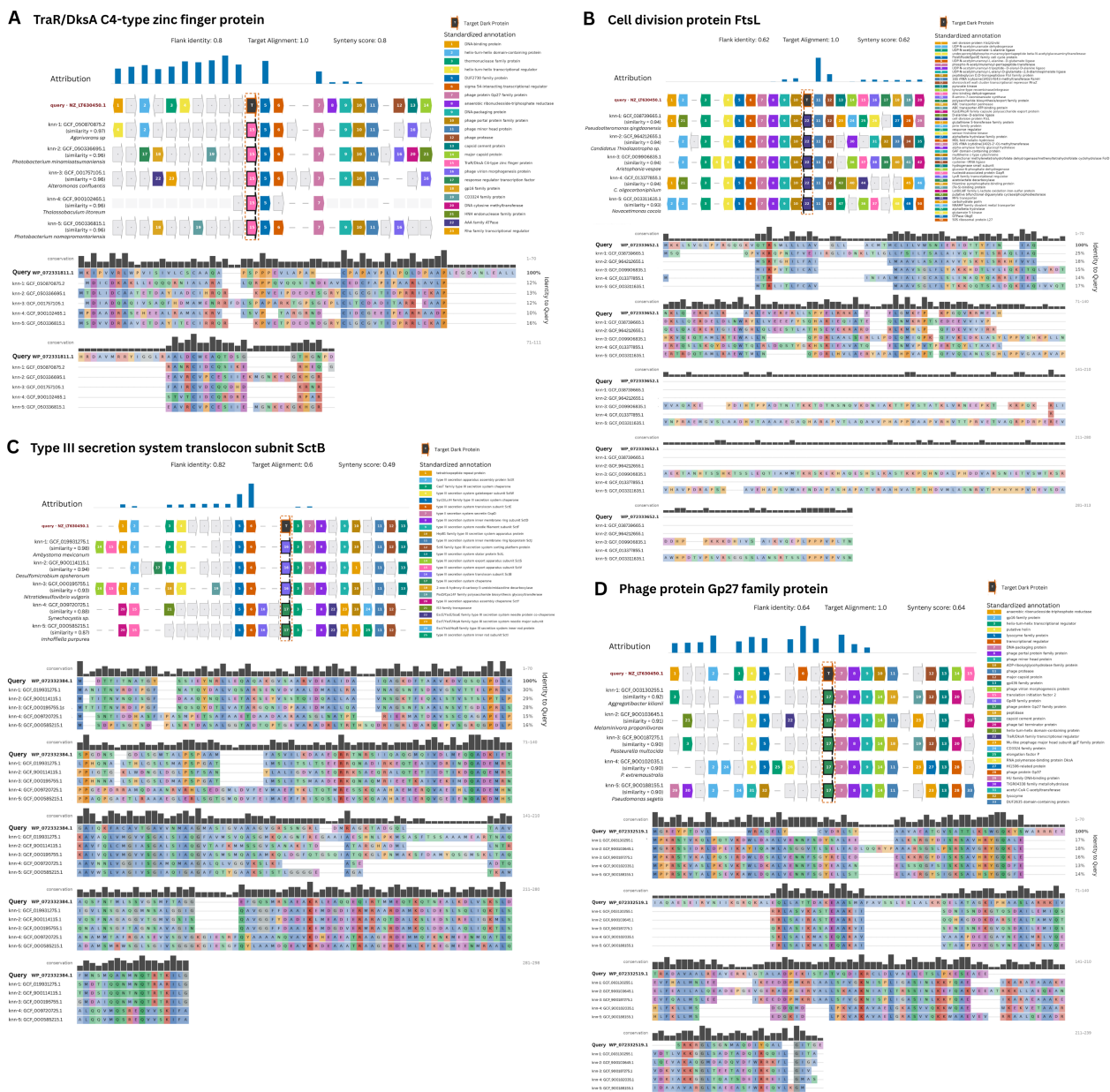
Figure S2. Multiple sequence alignment and Interpretation panels of Synnotate-annotated genes. (A) TraR/DksA C4-type zinc finger protein. (B) Cell division protein FtsL. (C) Type III secretion system translocon subunit SctB. (D) Phage protein Gp27 family protein. Protein multiple sequence alignments were generated using MAFFT 33 and visualized with pyMSAviz 34 .
