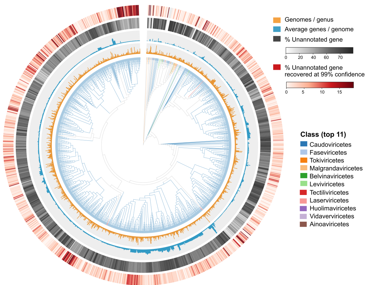
Figure S4. Distribution of dark proteome and Synnotate-annotated genes across viral genera.
