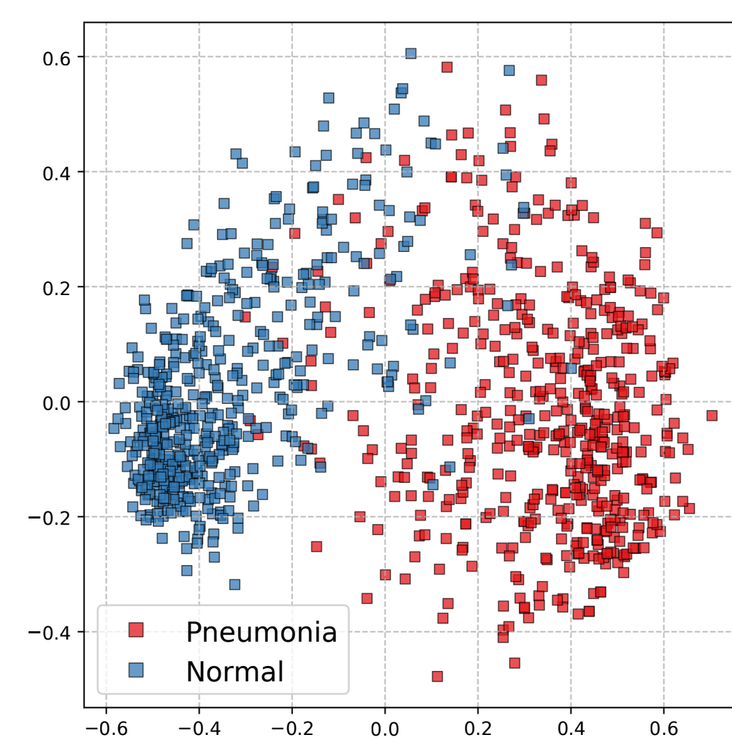
Figure 6. PCA visualization (2 components) of vision encoder features from MedCLIP, BioMedCLIP, and ENTRepCLIP. The row shows the feature distributions of medical VLMs with different variants: vanilla, w/ AT (Adversarial Training) and w/ SSL (Self-Supervised Learning)
