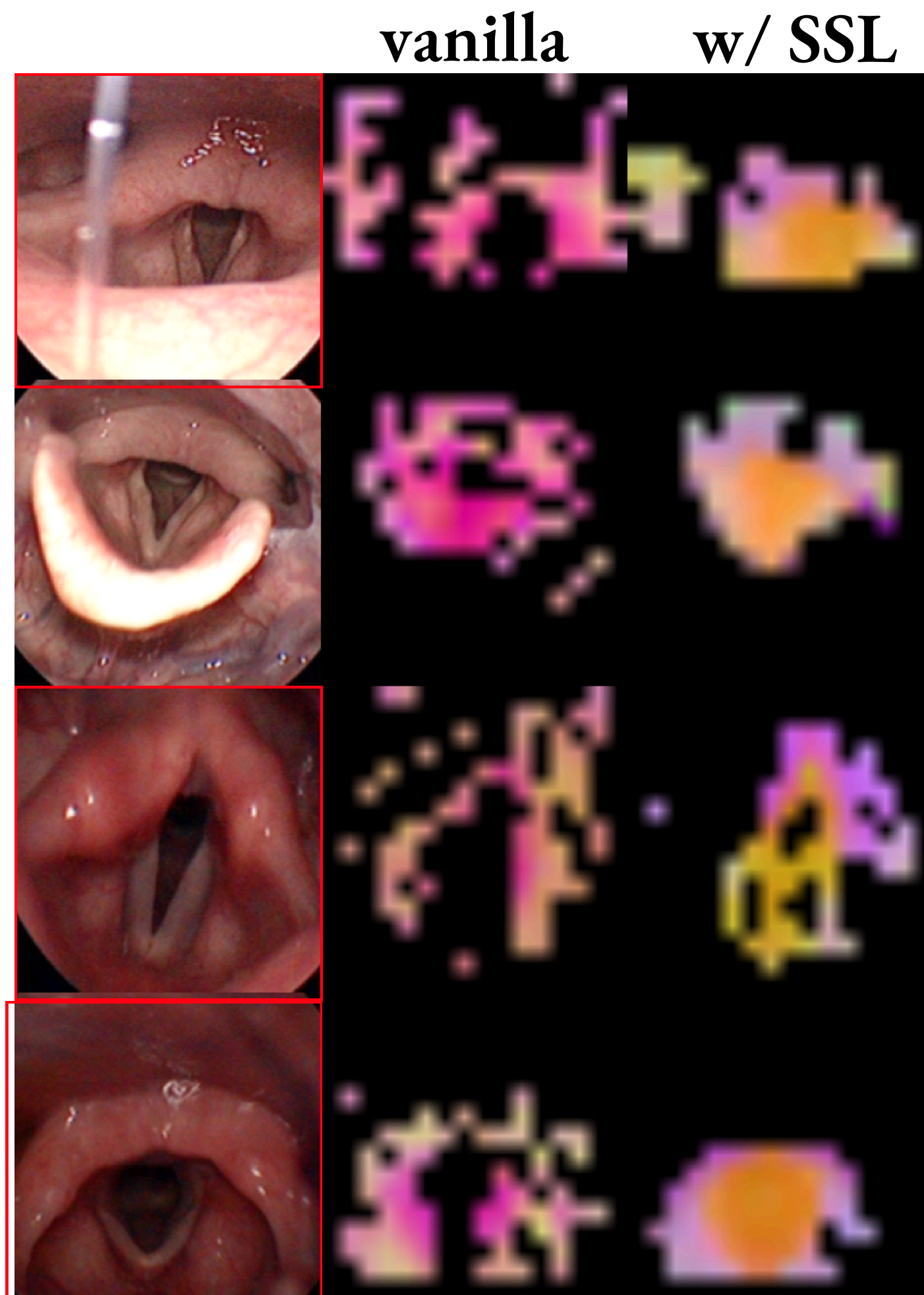
Figure 9. Visualization of feature representations of ENTRepCLIP using PCA projection with three components on four images from the vocal throat class. Images with red borders denote adversarial images created by adding Gaussian noise, while images without borders correspond to clean samples. The first PCA component is used to filter out background variations.
