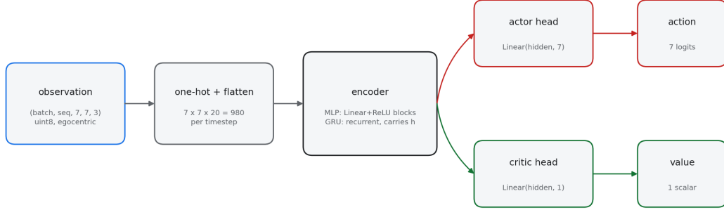
Figure 1: Top: MiniGrid-MemoryS17Random-v0. A cue (key or ball) sits in the west room; the corridor forks into a T with a key at one prong and a ball at the other, and success requires reaching the prong matching the cue. The agent spawns at a random corridor position facing away from the cue, so the information must be actively sought. Bottom: one shared encoder feeding a linear actor head over the 7 actions and a linear critic head. The encoder is the only part that differs between arms.
