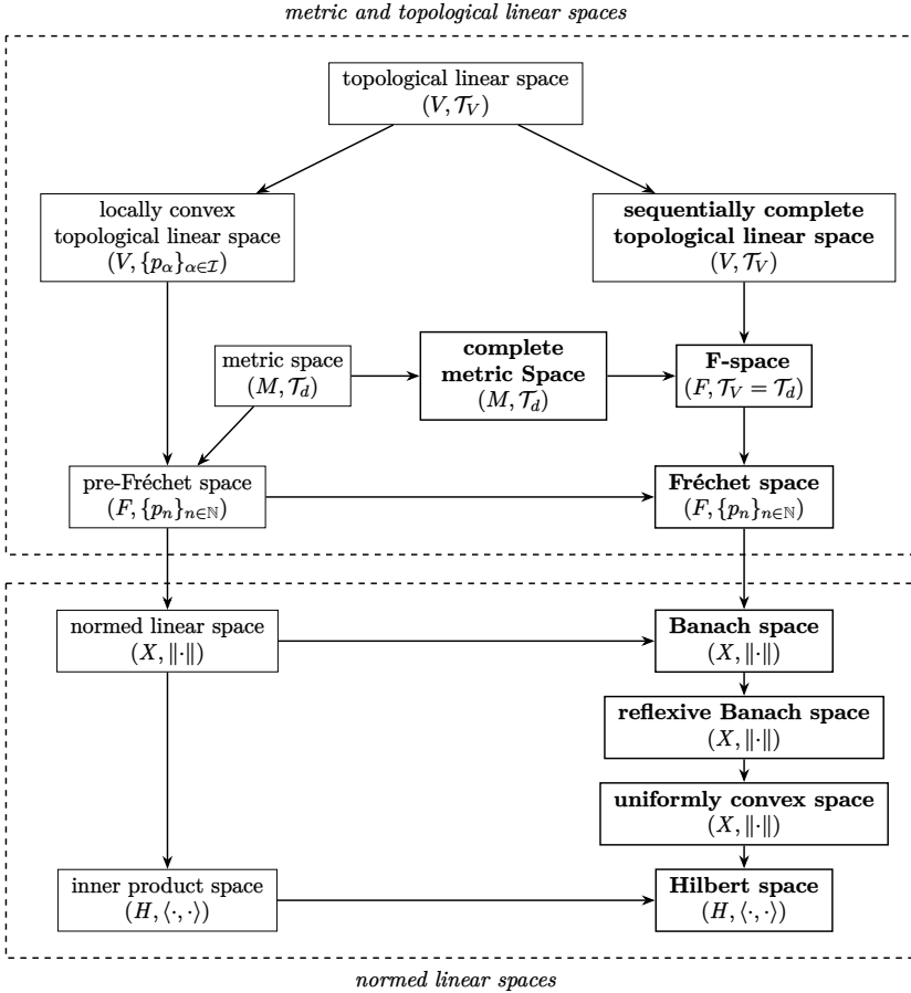
Figure 5.1: The hierarchy of metric and topological linear spaces
