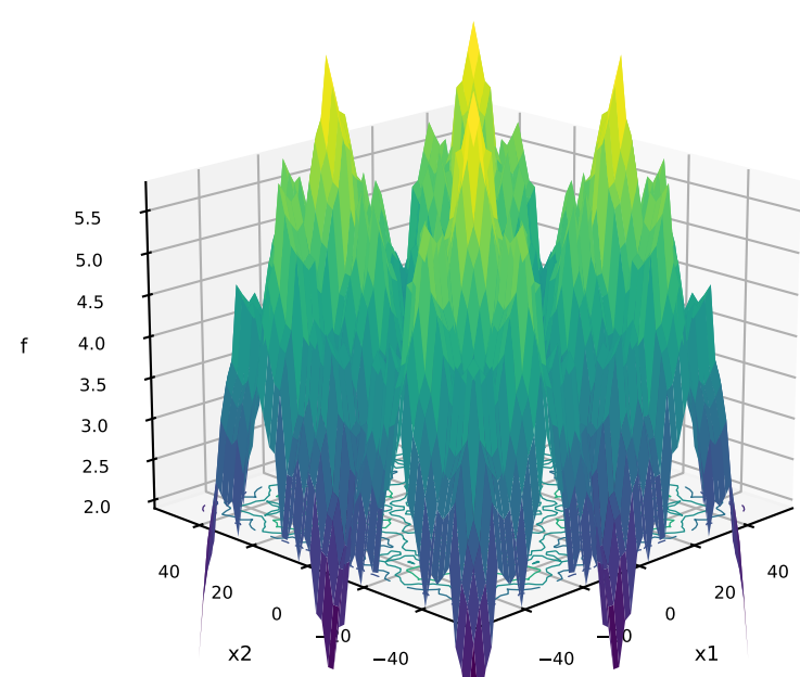
19: Gallagher21
