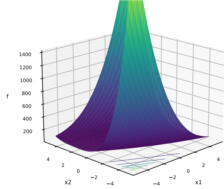
22: Zakharov
