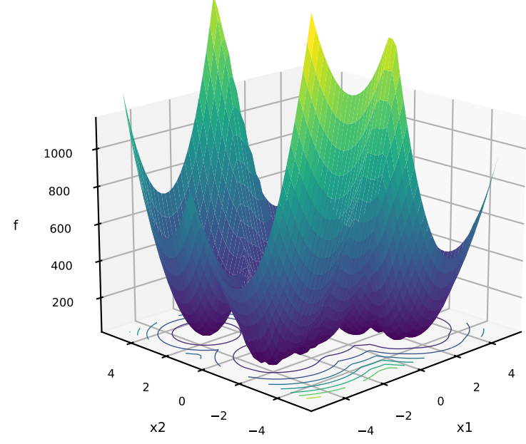
23: Levy
