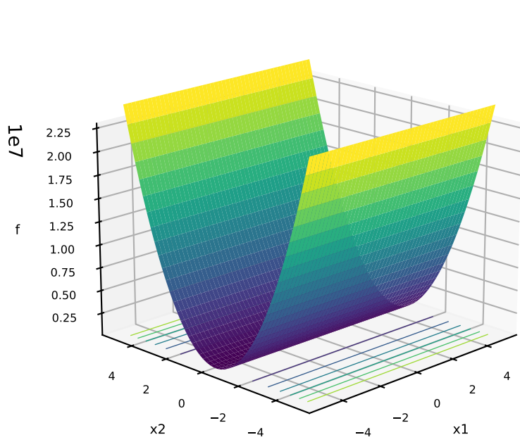
6: AttractiveSector
