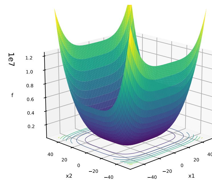
32: Quartic
