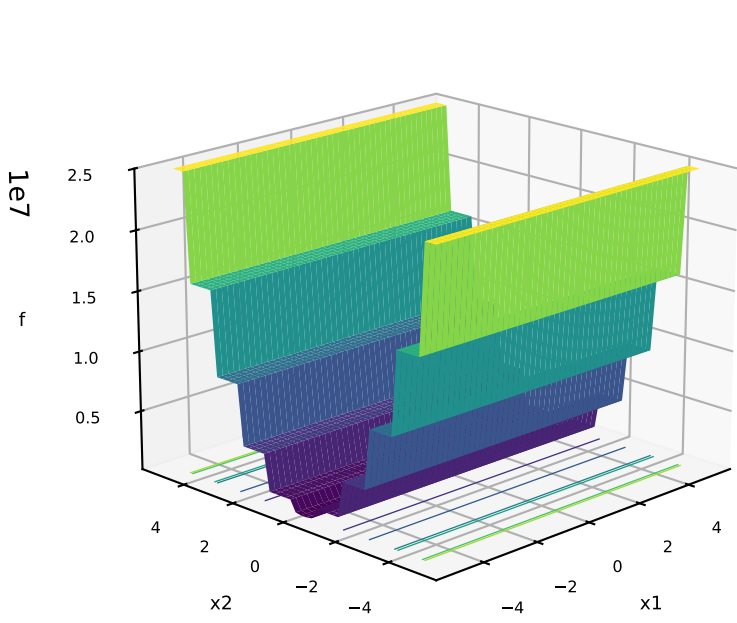
11: Rastrigin
