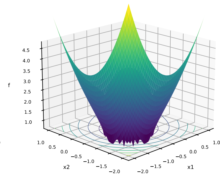
32: Quartic
