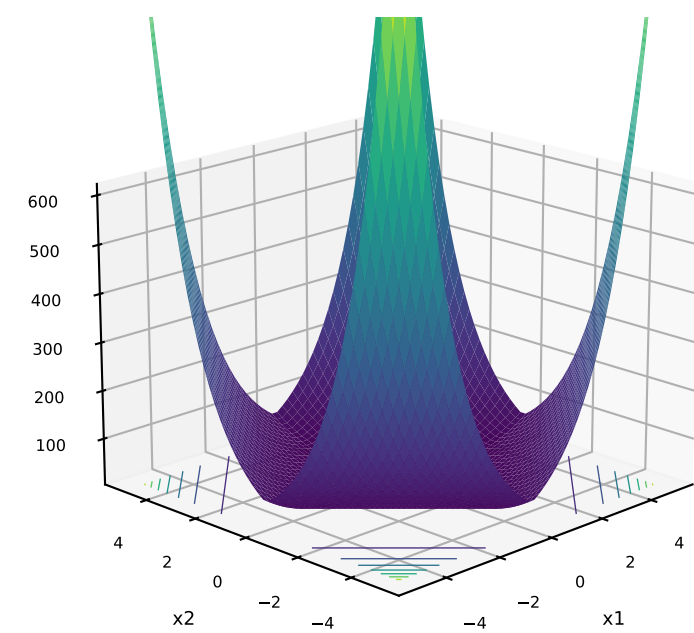
29: HCF
