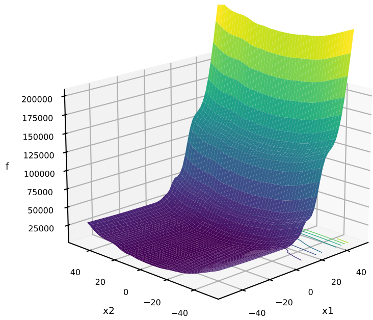
8: StepRastrigin
