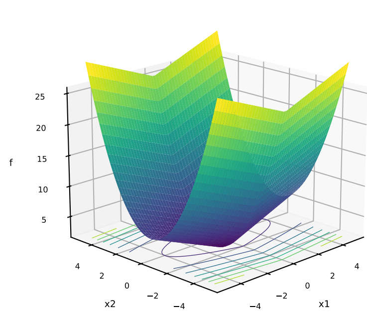
7: StepEllipsoidal
