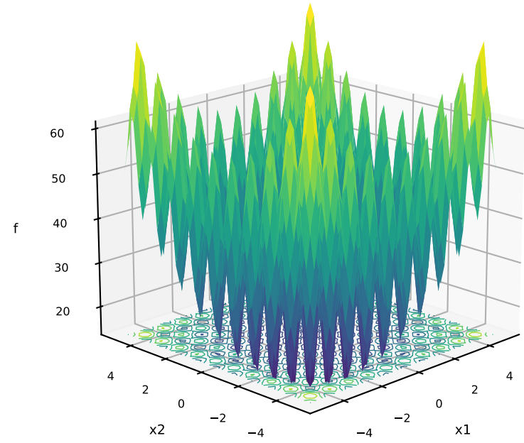
15: Weierstrass
