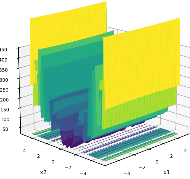
21: LunacekBiRastrigin
