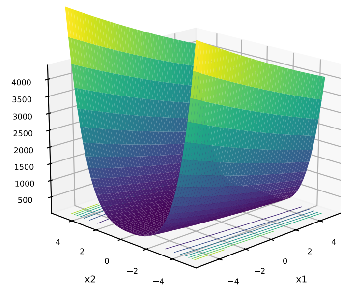
29: HCF
